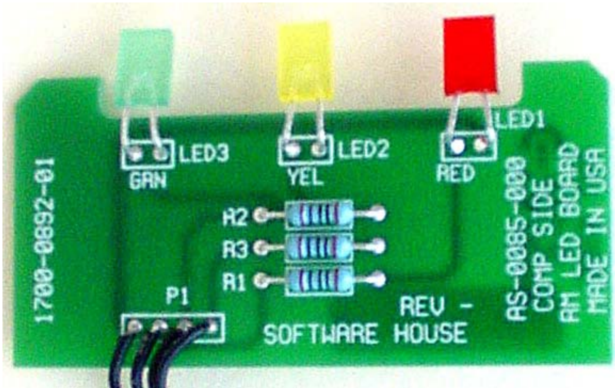
LED Board Front
