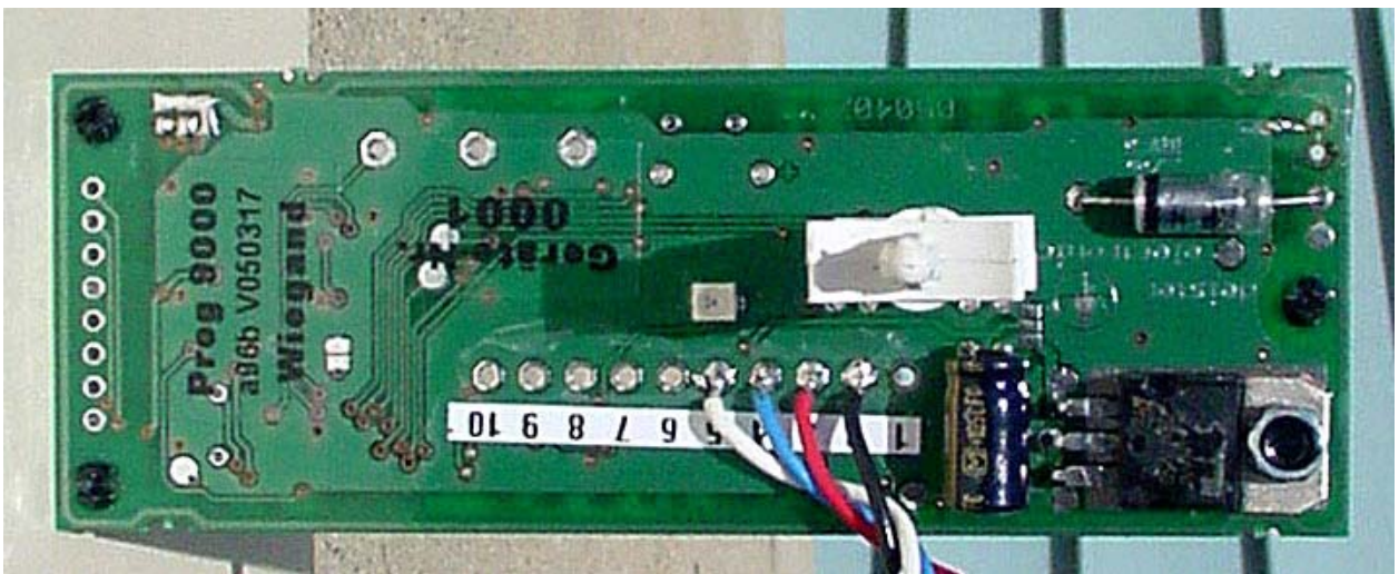
Antenna Drive Board Rear
