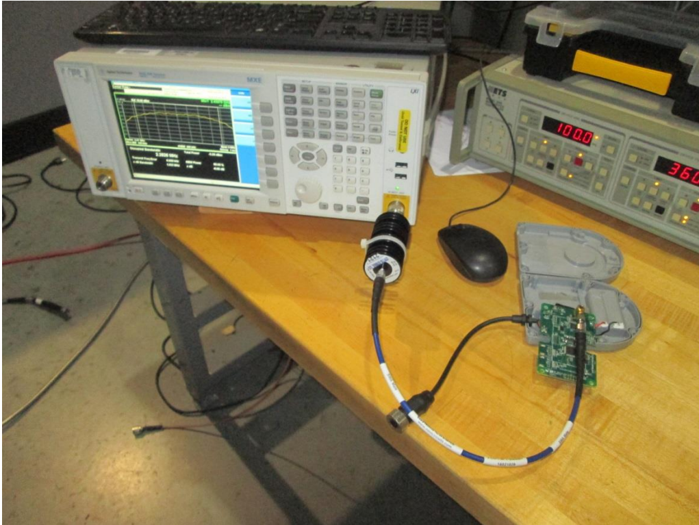
Conducted Emission at the Antenna Port (Setup Overview)
