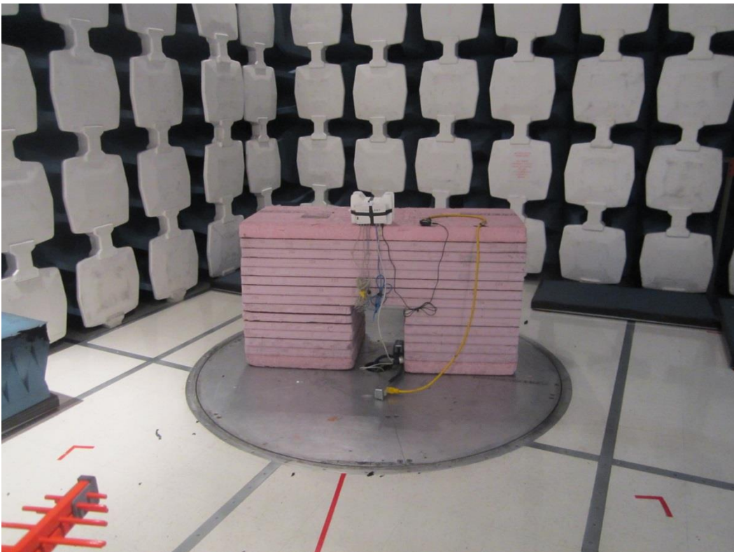
30MHz – 1GHz (EUT in Y orientation – EUT antenna vertical)
