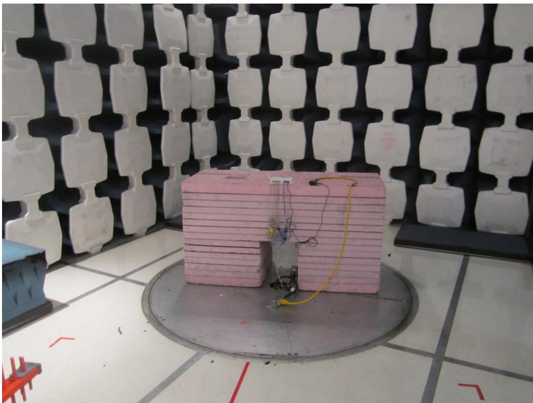
30MHz – 1GHz (EUT in X orientation – EUT antenna vertical)
