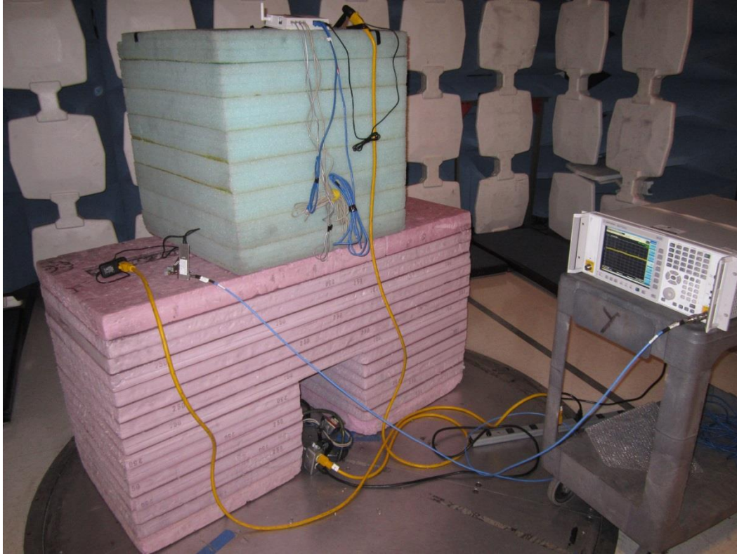
18GHz-25GHz (worst case orientation)
