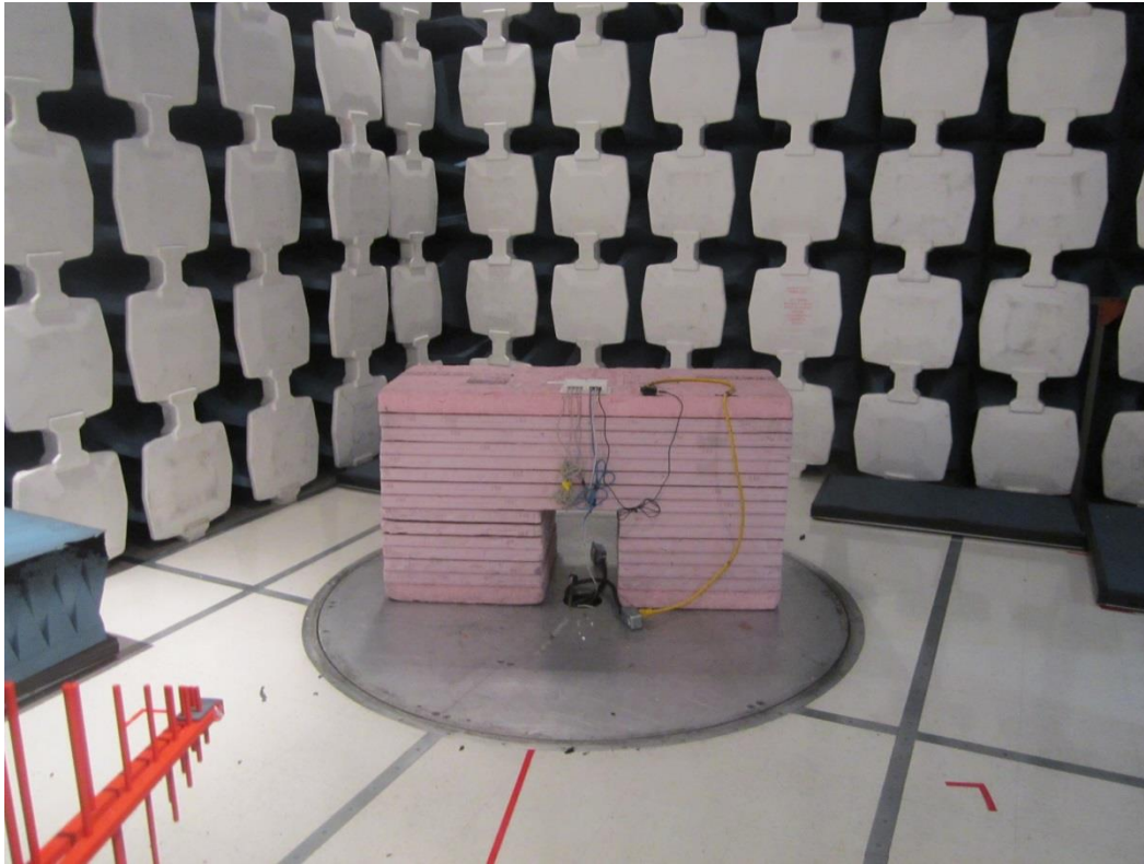
30MHz – 1GHz (EUT in X orientation – EUT antenna horizontal)
