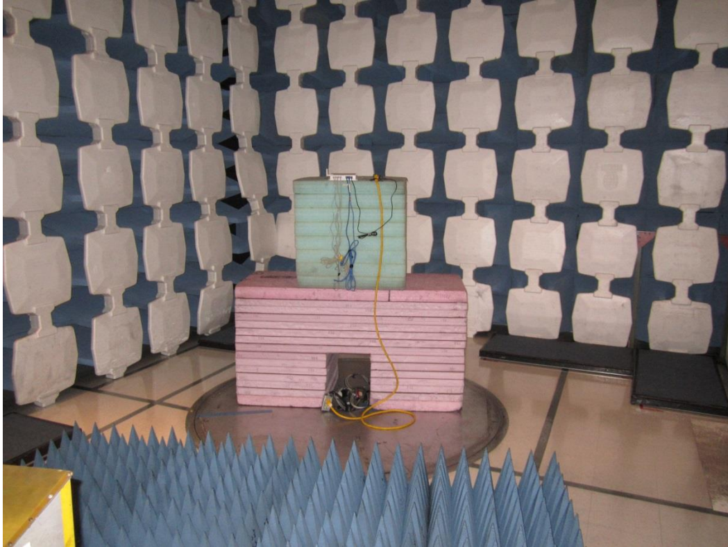
1GHz – 6GHz (worst case orientation)
