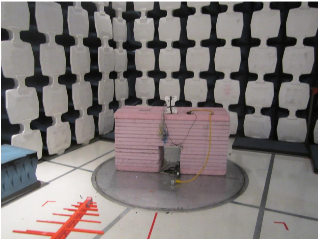
30MHz – 1GHz (EUT in Z orientation – EUT antenna vertical)
