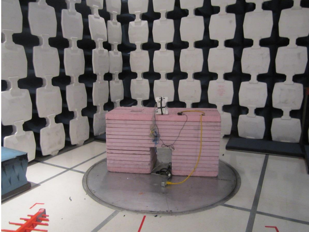
30MHz – 1GHz (EUT in Z orientation – EUT antenna horizontal)
