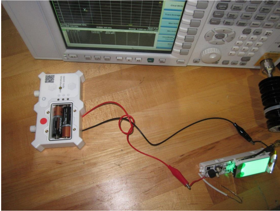
Bluetooth LE Kitchen Thermometer, Antenna Port Measurement
