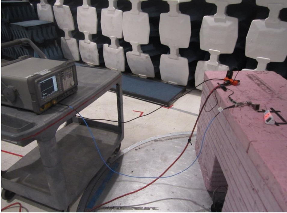
Bluetooth LE Kitchen Thermometer, Radiated Emissions 18-25 GHz
