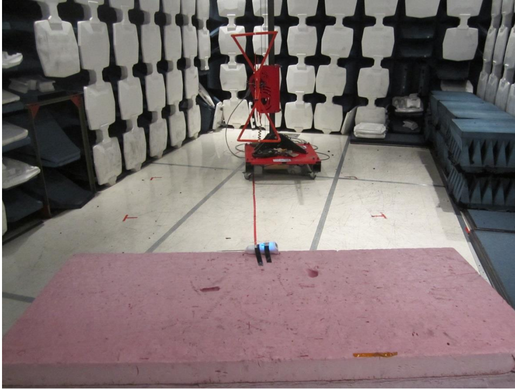
30-1000 MHz, EUT to Antenna
