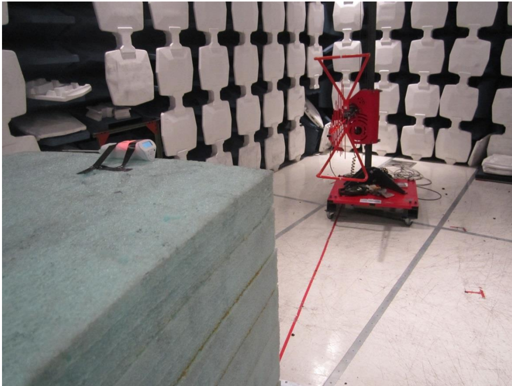
30-1000 MHz REMI Test, EUT to Antenna Close
