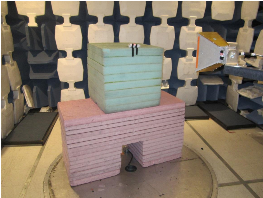
1-6 GHz REMI Test, Antenna to EUT
