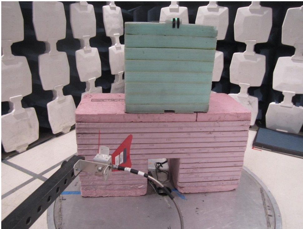
Bluetooth LE Kitchen Thermometer, Radiated Emissions 1-18 GHz
