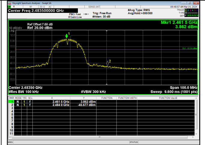
IEEE 802.11g / High Channel
