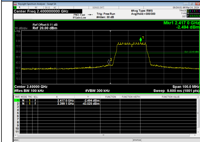
IEEE 802.11n(HT20) / Low Channel
