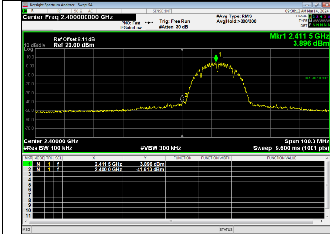
IEEE 802.11g / Low Channel
