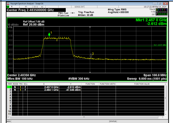
IEEE 802.11n(HT20) / High Channel
