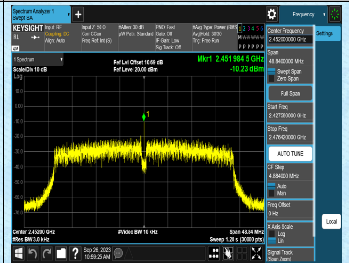
11N40SISO-Ant1-2452
