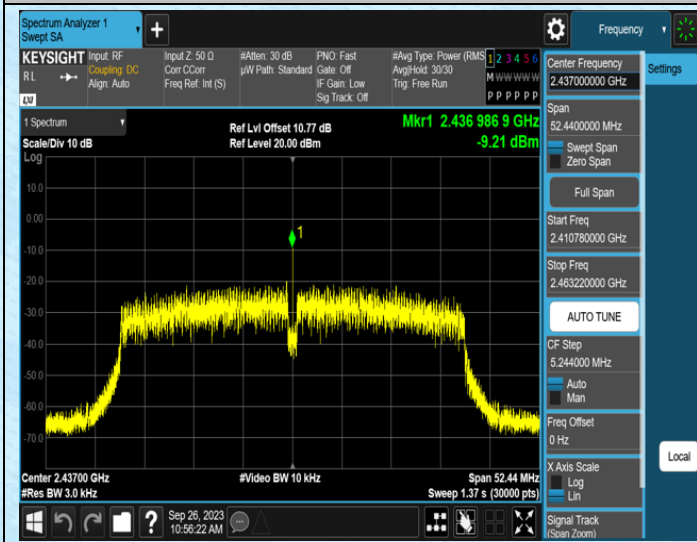
11N40SISO-Ant1-2437
