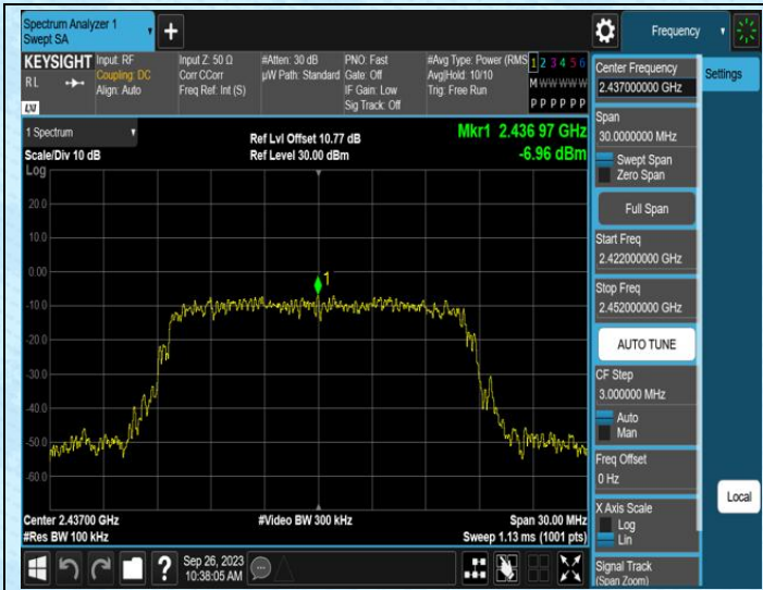
11G-Ant1-2437-0-Reference
