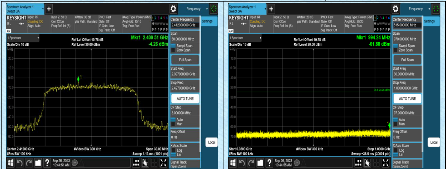
11N20SISO-Ant1-2412-0~Reference
