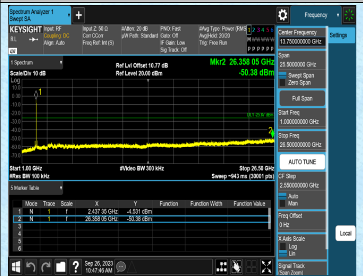
11N20SISO-Ant1-2437-1000~26500
