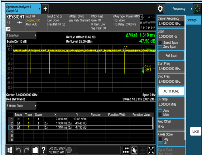
NTVN-11N20SISO-Ant1-2462
