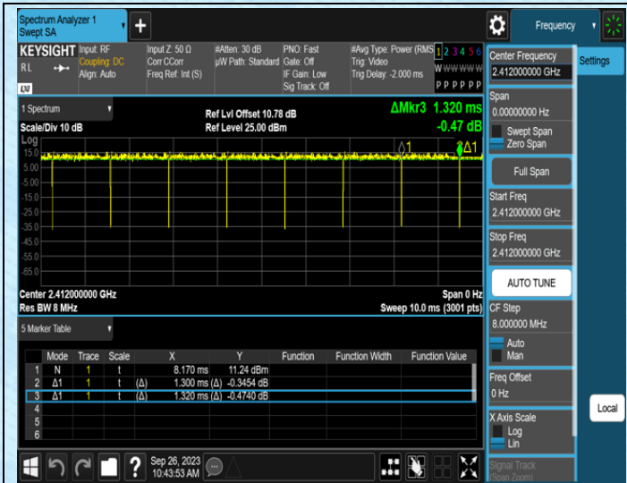
NTVN-11N20SISO-Ant1-2412
