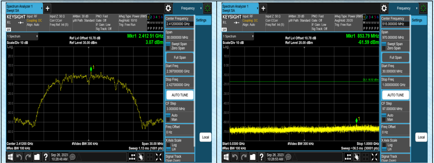
11B-Ant1-2412-0-Reference
