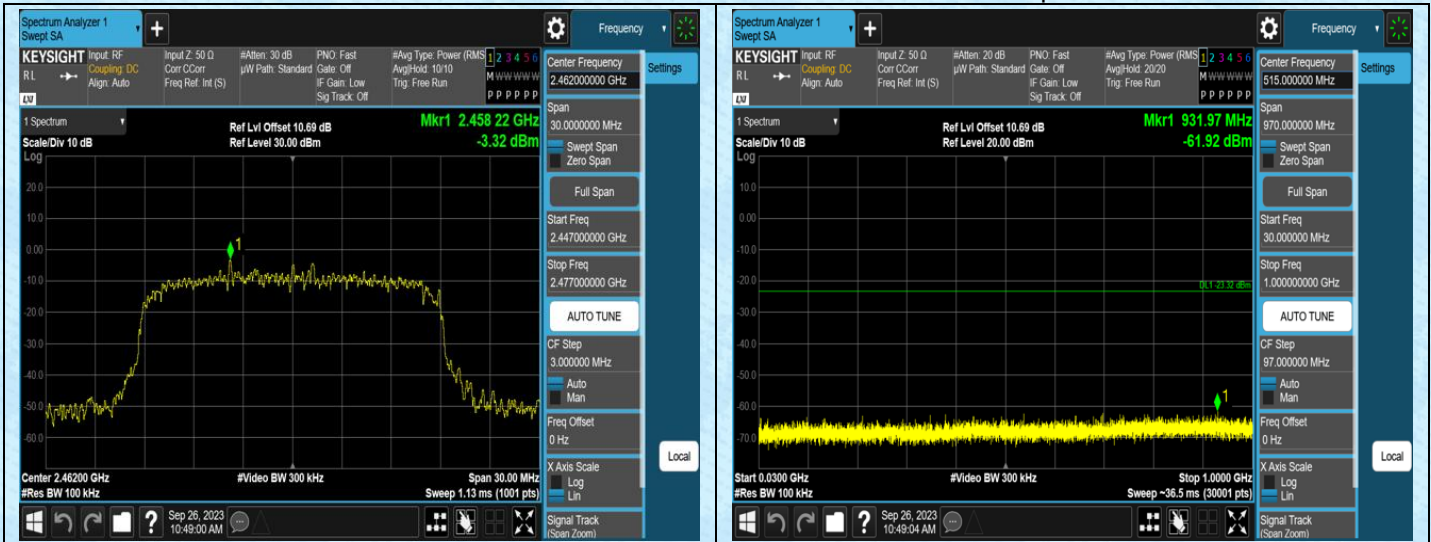
11N20SISO-Ant1-2462-0~Reference
