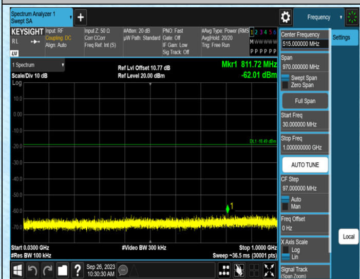
11B-Ant1-2437-30-1000
