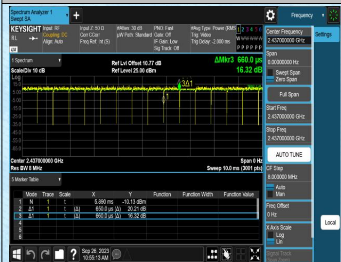
NTVN-11N40SISO-Ant1-2437
