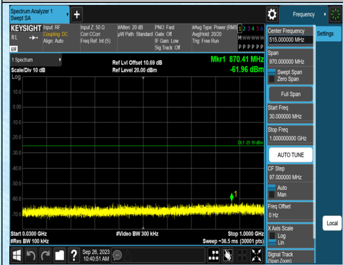
11G-Ant1-2462-30-1000
