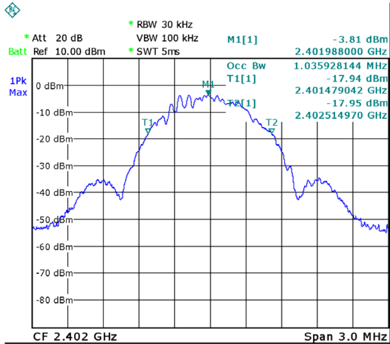
BLE: channel 0
