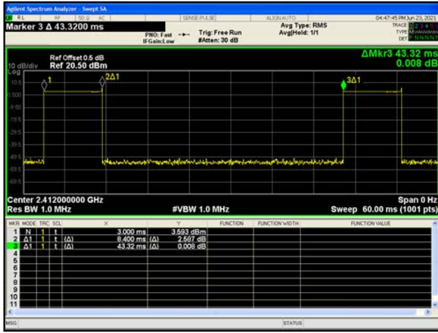
Wi-Fi 802.11b
