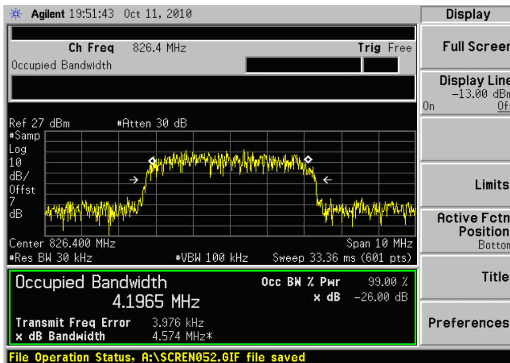
Channel 4132
