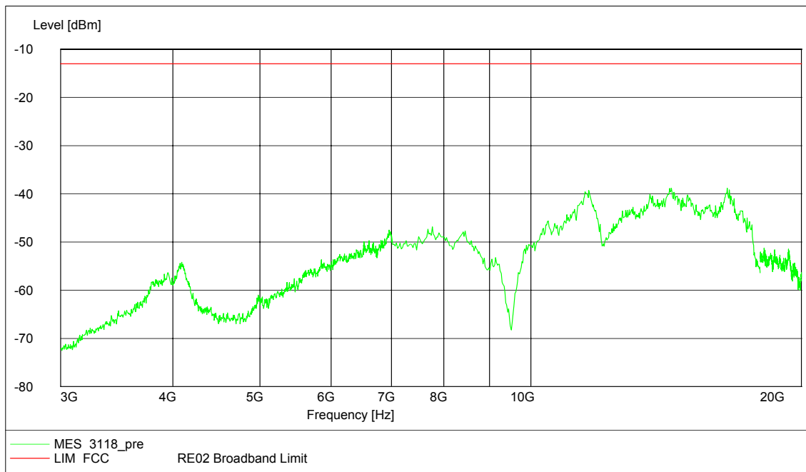
Channel 4183, 3GHz~20GHz
