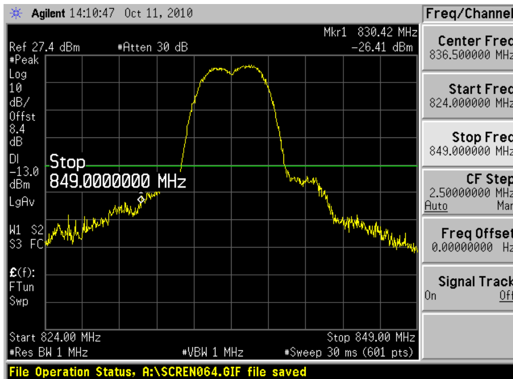
Channel 4183, 824MHz~849MHz
