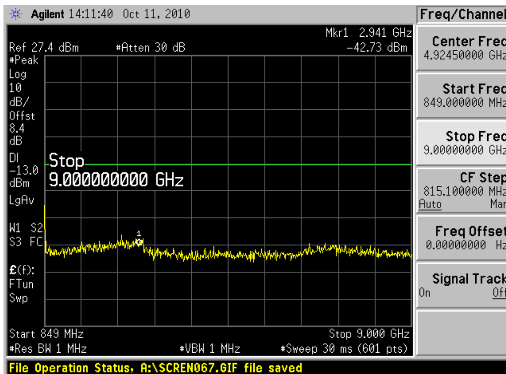
Channel 4183, 849MHz~9GHz
