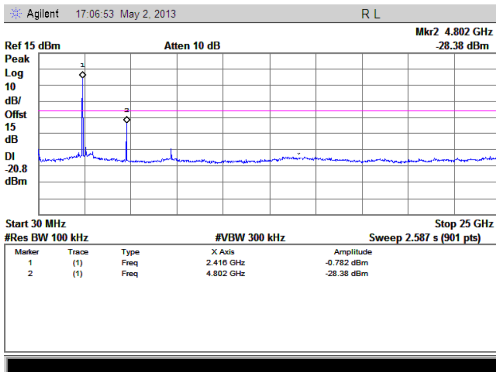
(Plot G.1: Channel = 0, 30MHz to 25GHz @ 8-DPSK)
