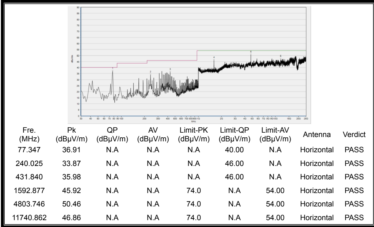
(30MHz to 25GHz, Antenna Horizontal @8-DPSK, channel 0)
