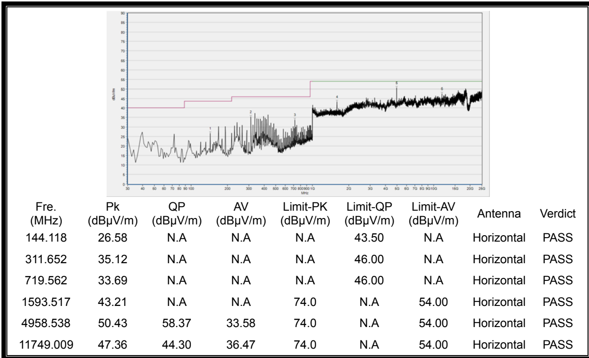
(30MHz to 25GHz, Antenna Horizontal @ GFSK, channel 78)
