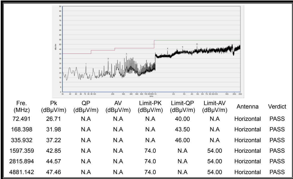
(30MHz to 25GHz, Antenna Horizontal @ π/4-DQPSK, channel 39)
