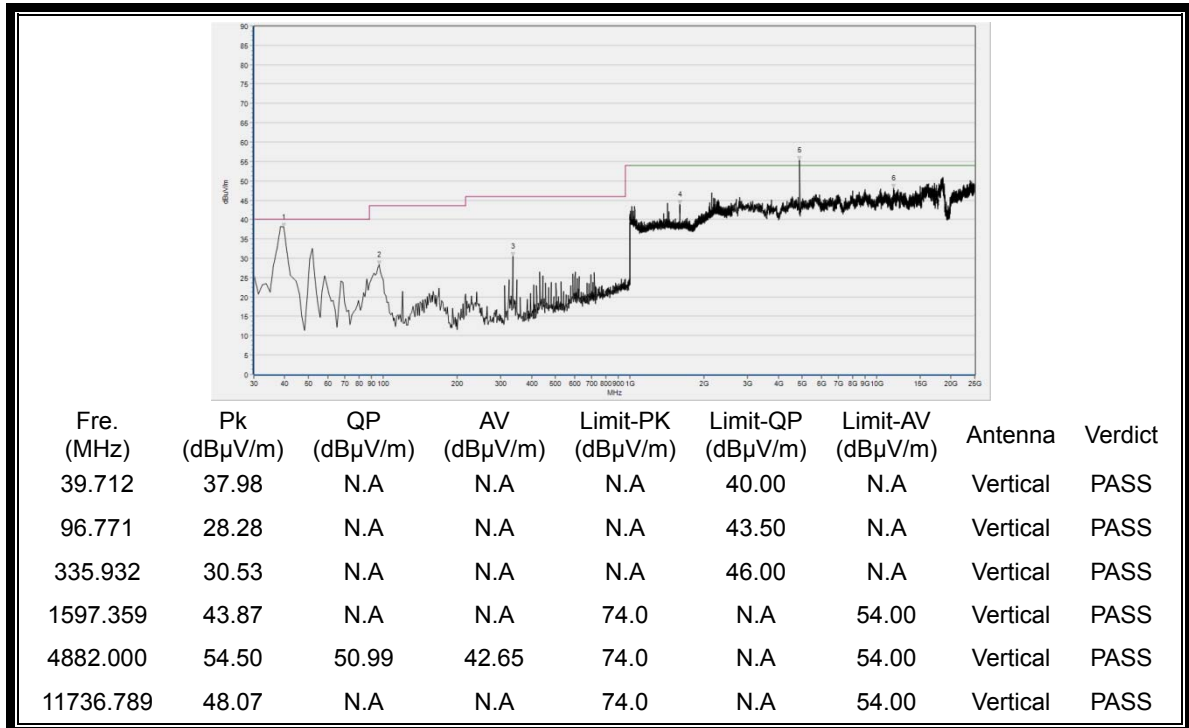
(30MHz to 25GHz, Antenna Vertical @ π/4-DQPSK, channel 39)
