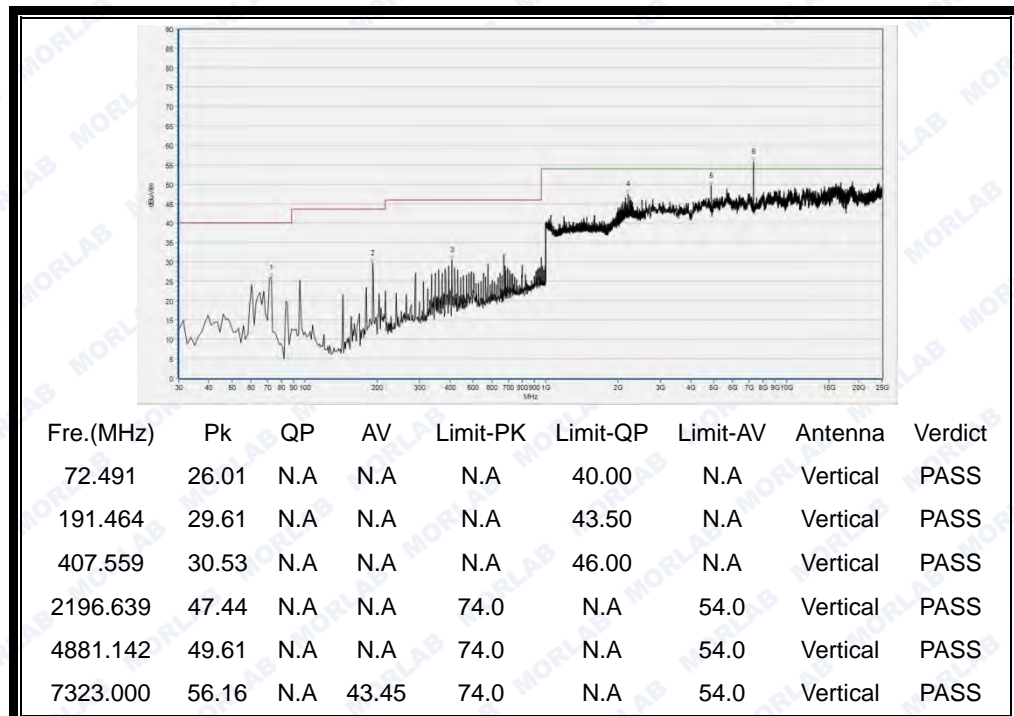
(30MHz to 25GHz, Antenna Vertical @ GFSK, channel 39)
