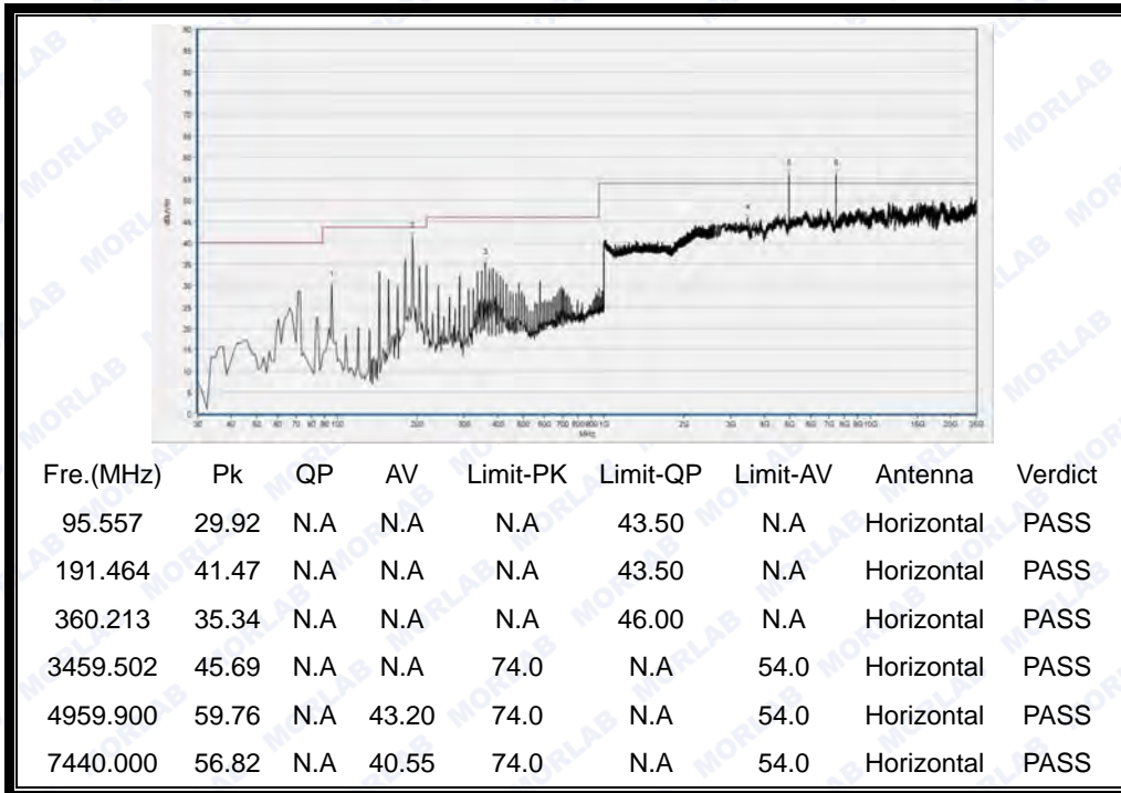
(30MHz to 25GHz, Antenna Horizontal @8-DPSK, channel 78)
