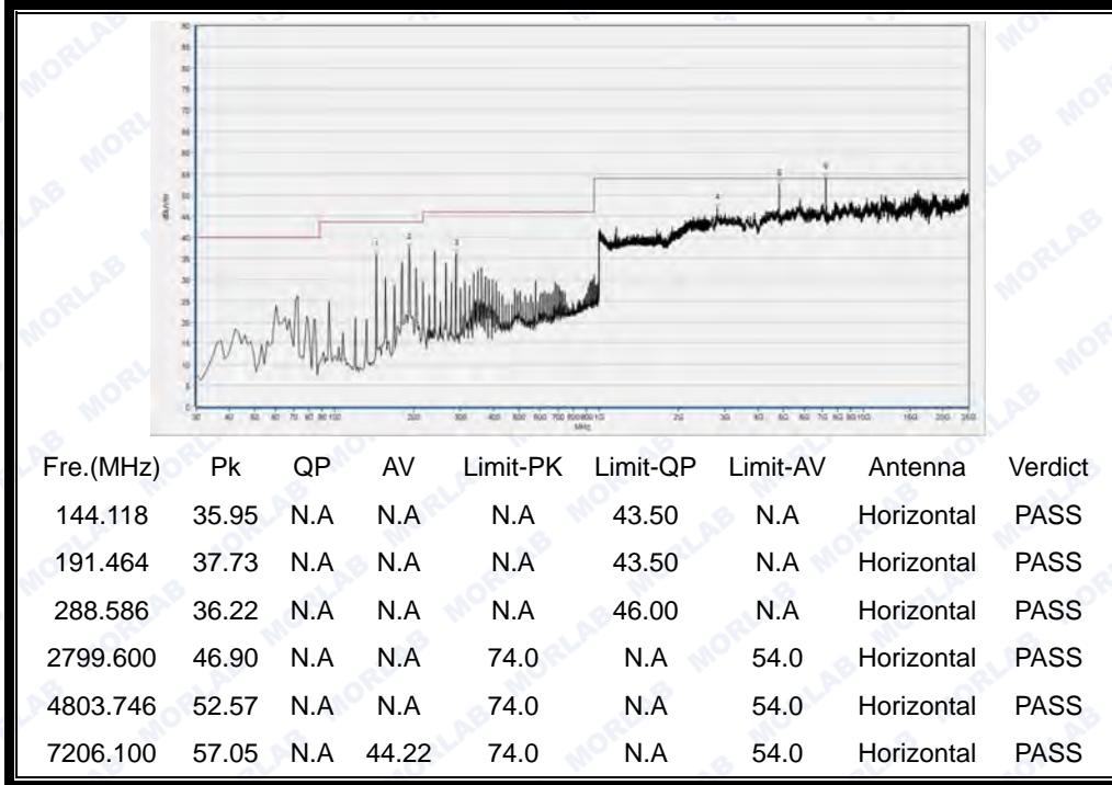
(30MHz to 25GHz, Antenna Horizontal @ GFSK, channel 0)
