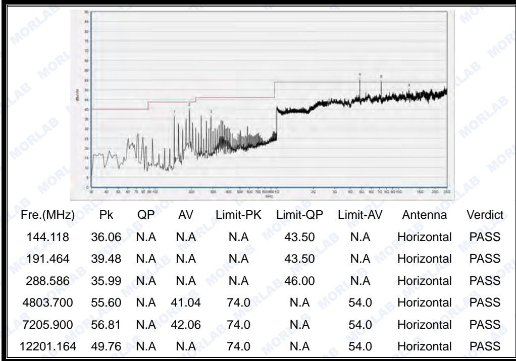
(30MHz to 25GHz, Antenna Horizontal @8-DPSK, channel 0)
