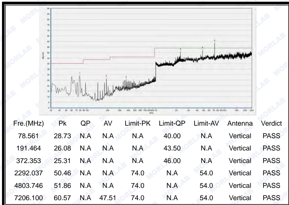
(30MHz to 25GHz, Antenna Vertical @ GFSK, channel 0)
