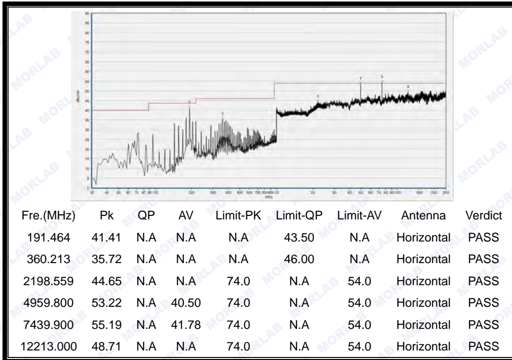
(30MHz to 25GHz, Antenna Horizontal @ GFSK, channel 78)
