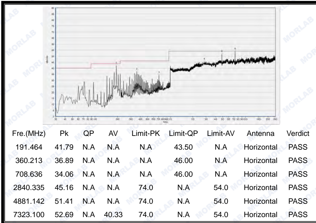
(30MHz to 25GHz, Antenna Horizontal @ GFSK, channel 39)
