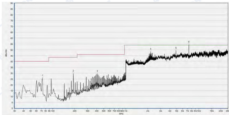
(30MHz to 25GHz, Antenna Horizontal @8-DPSK, channel 39)
