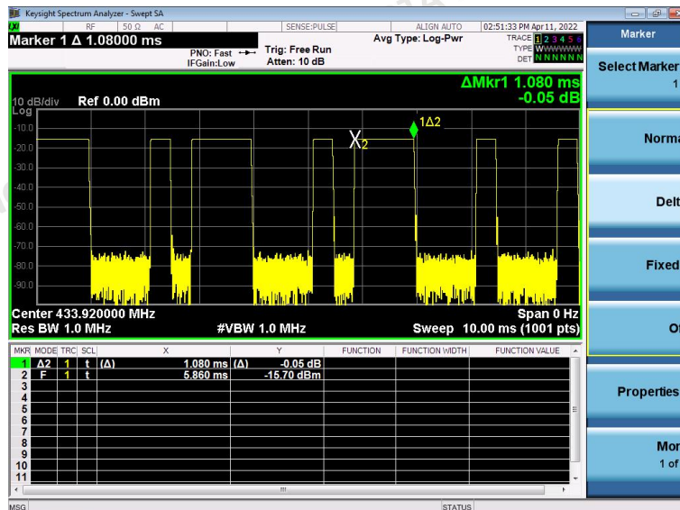
(Time per burst: 1.080ms*23pcs)
