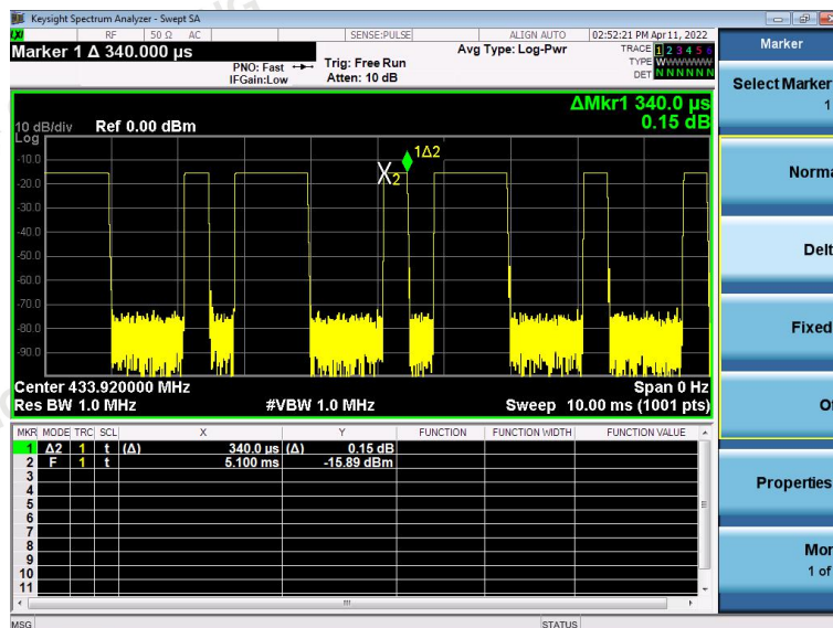
(Time per burst: 0.340ms*23pcs)
