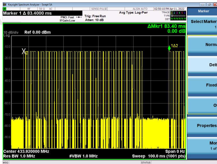
(Transmit cycle 83.40ms)
