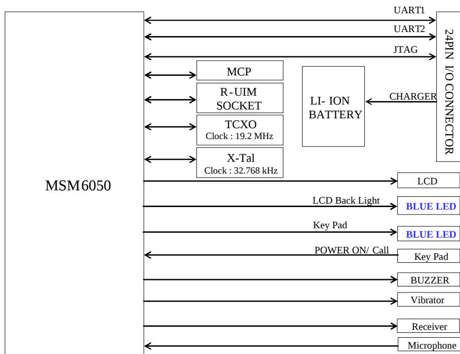
BCL862S Logic Part Block Diagram
