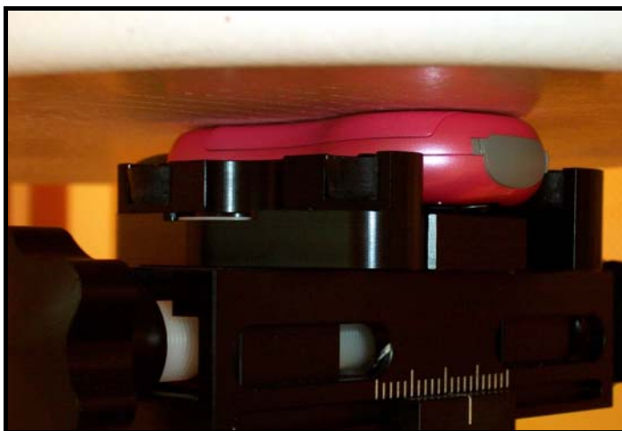
Figure 9.5 Muscle SAR Test Setup -- Touch Position --
