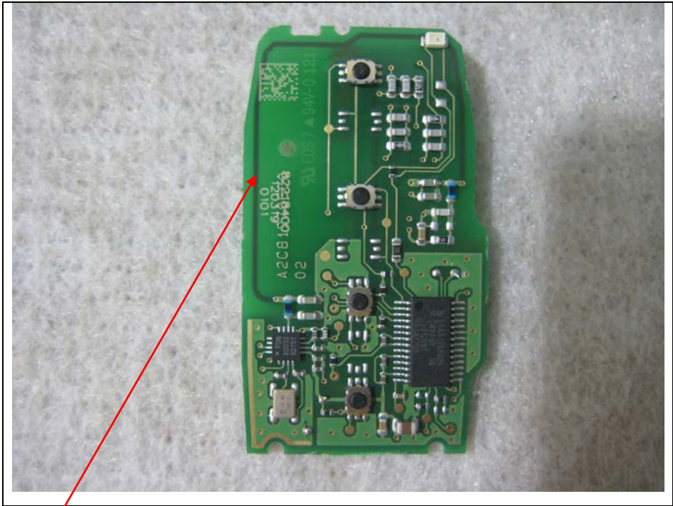
PCB Pattern Antenna
