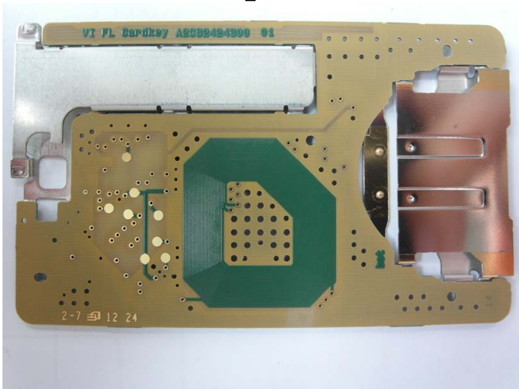
< PCB_Bottom >
