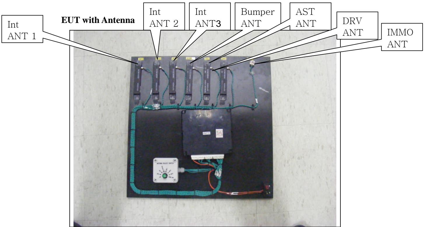
Front View of EUT
