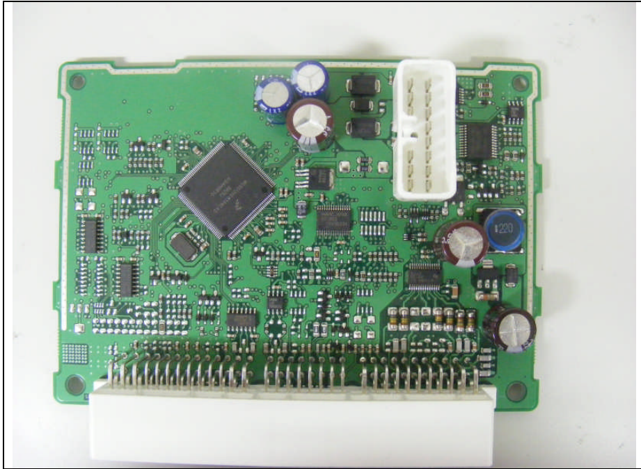
Top View of Main-board
