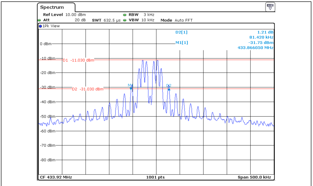
20 dB Bandwidth
