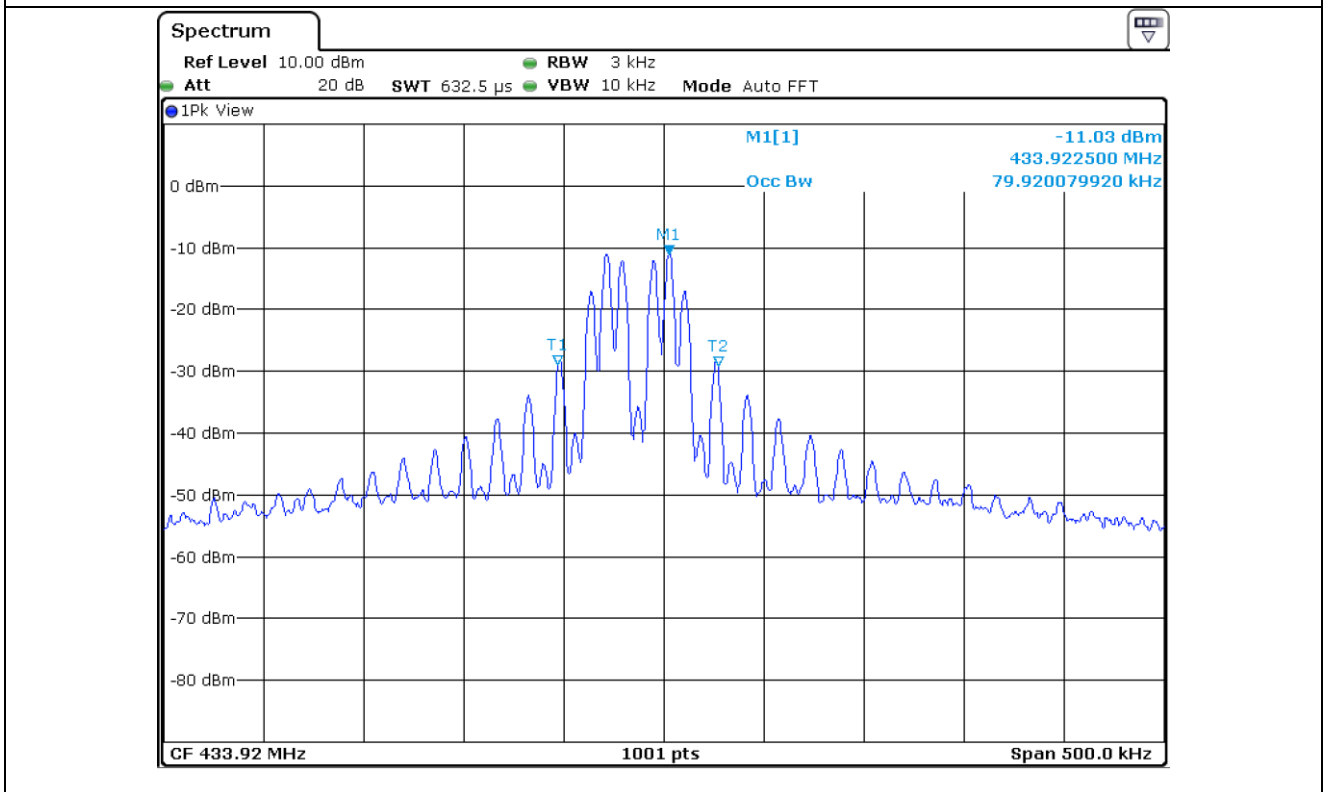
99% Bandwidth
