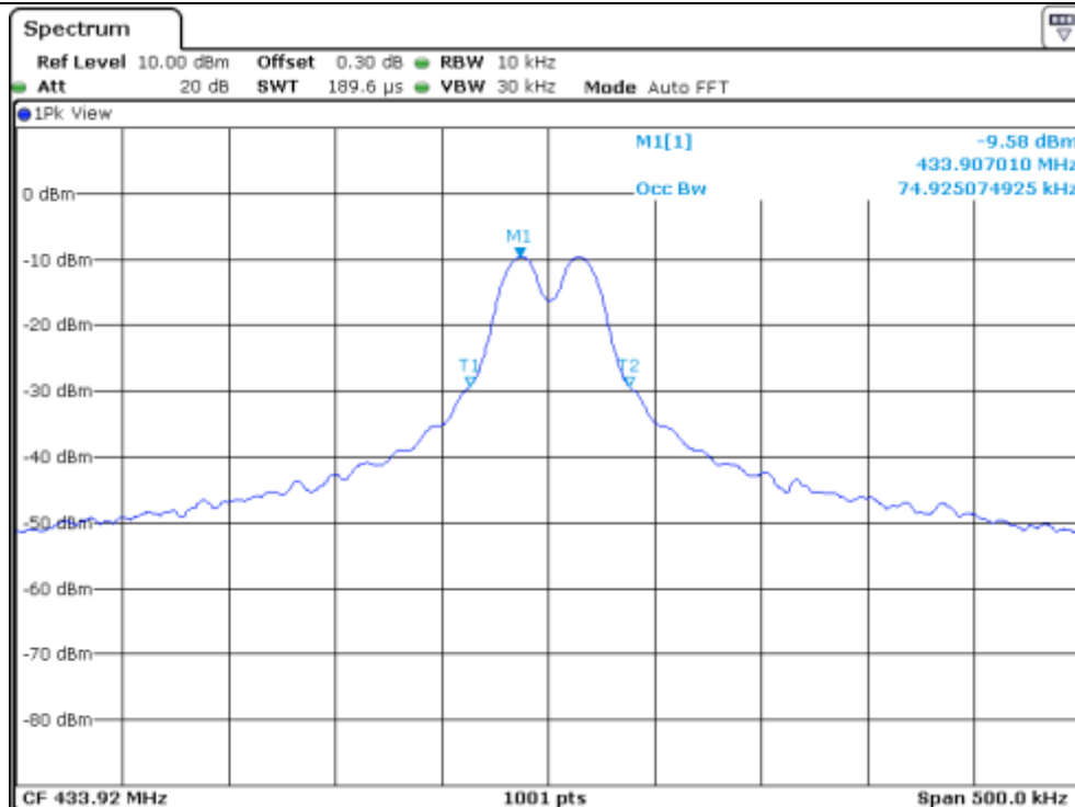
20 dB Bandwidth
