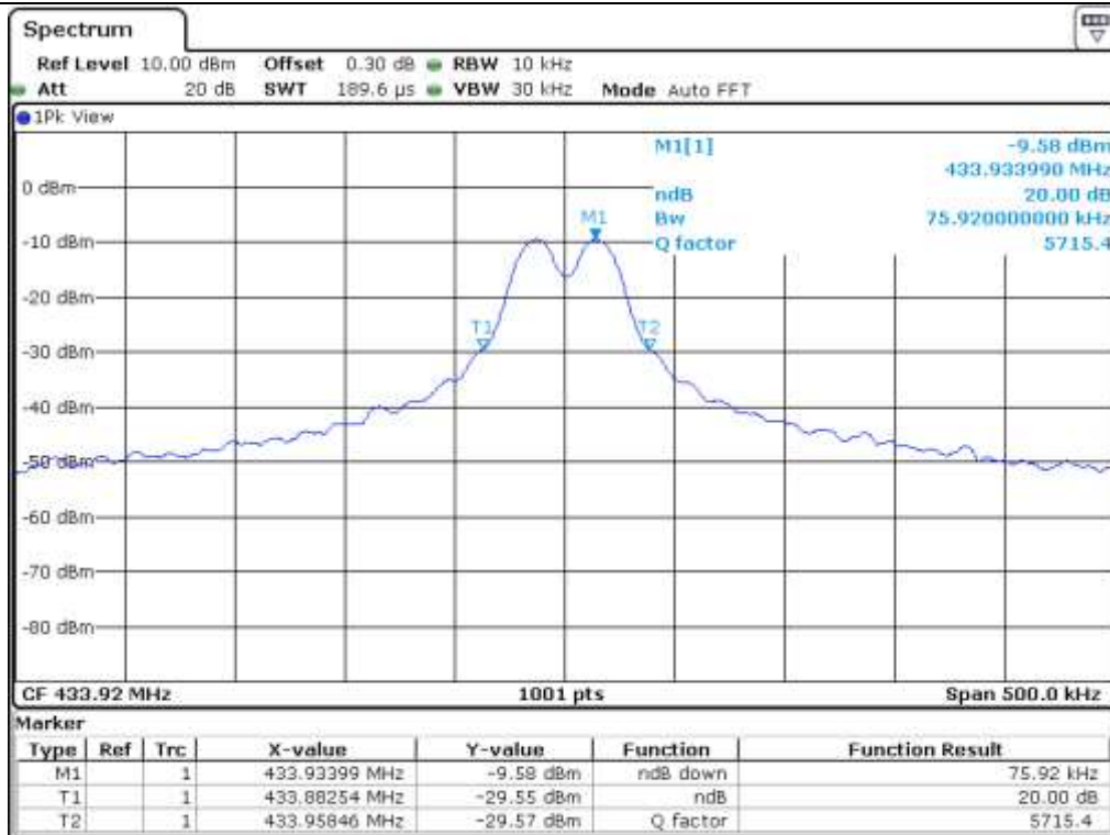
20 dB Bandwidth
