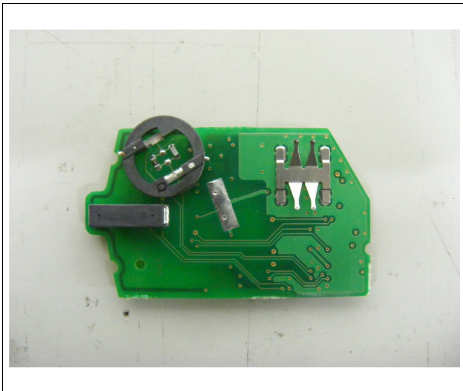
Bottom View of Main-board
