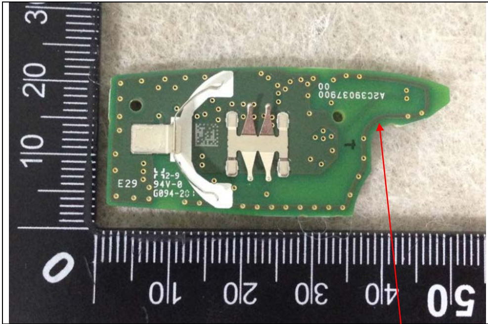
PCB Antenna
