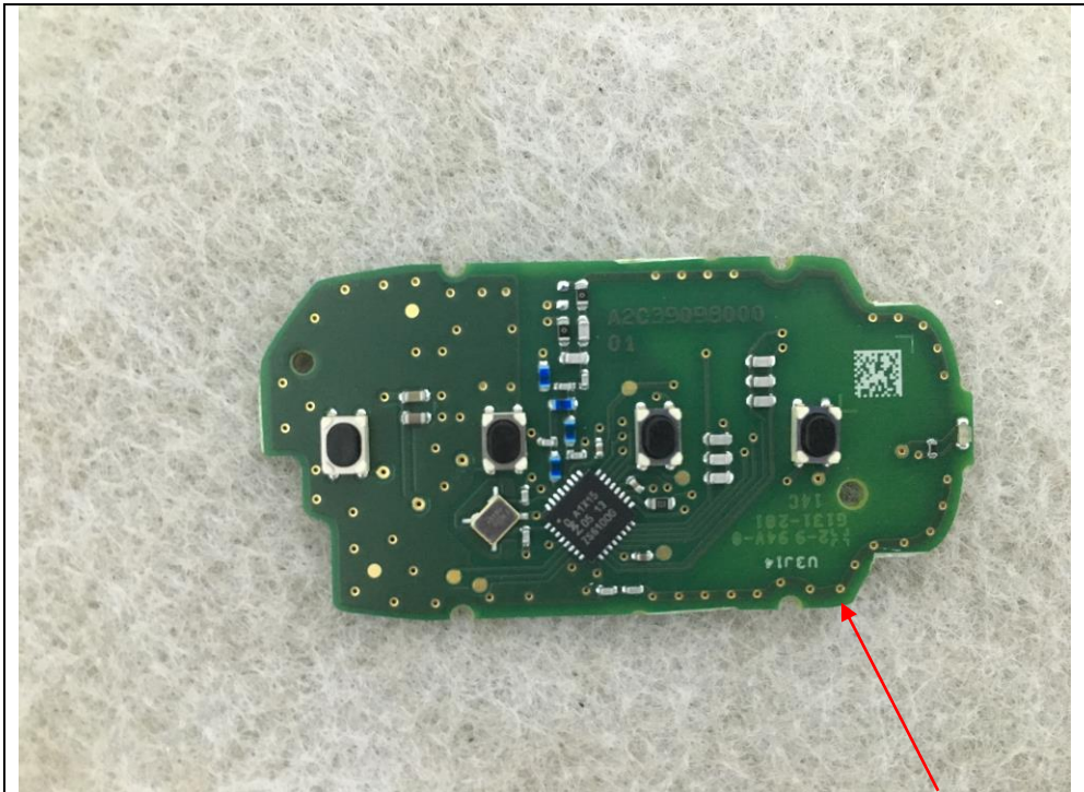
PCB Antenna
