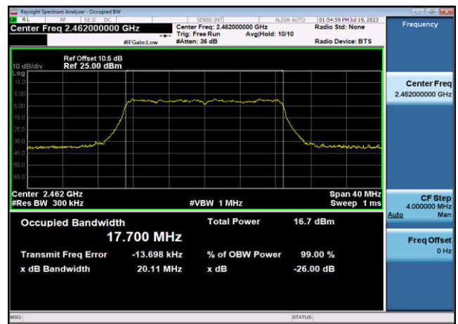
99% Bandwidth-802.11n(HT20),2462MHz ,Ant2
