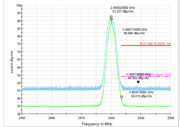
Test Mode: \pi/4 DQPSK-High Hopping-off
