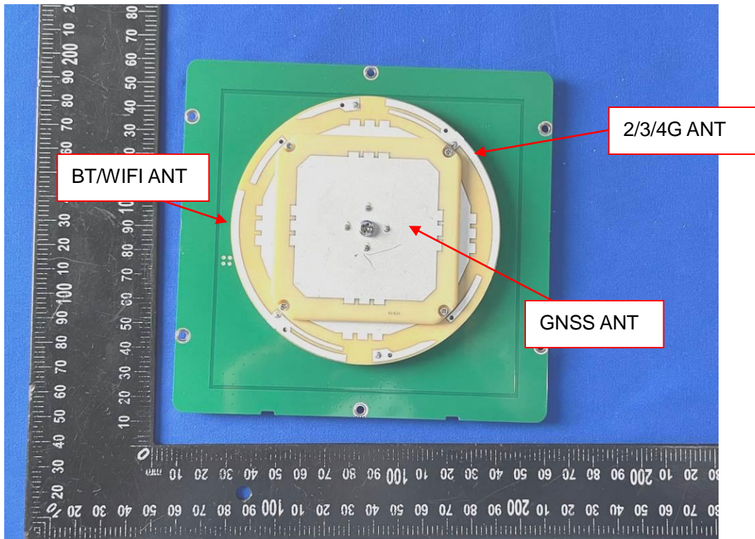
Internal view(PA-3 Plus)
