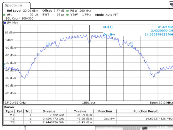
OBW NVNT b 2437MHz Ant1
