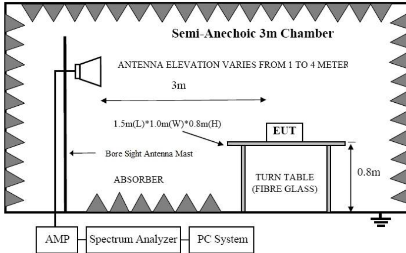
Above 1GHz Test Setup
