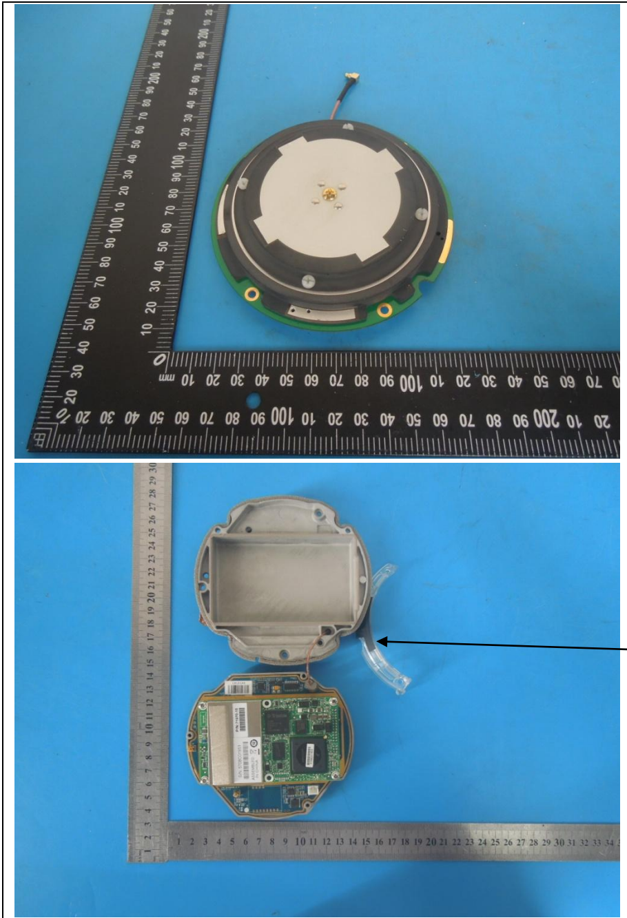
2G/3G Antenna
