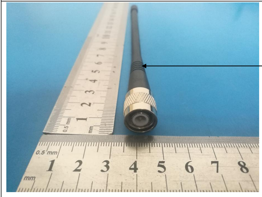
UHF Antenna
