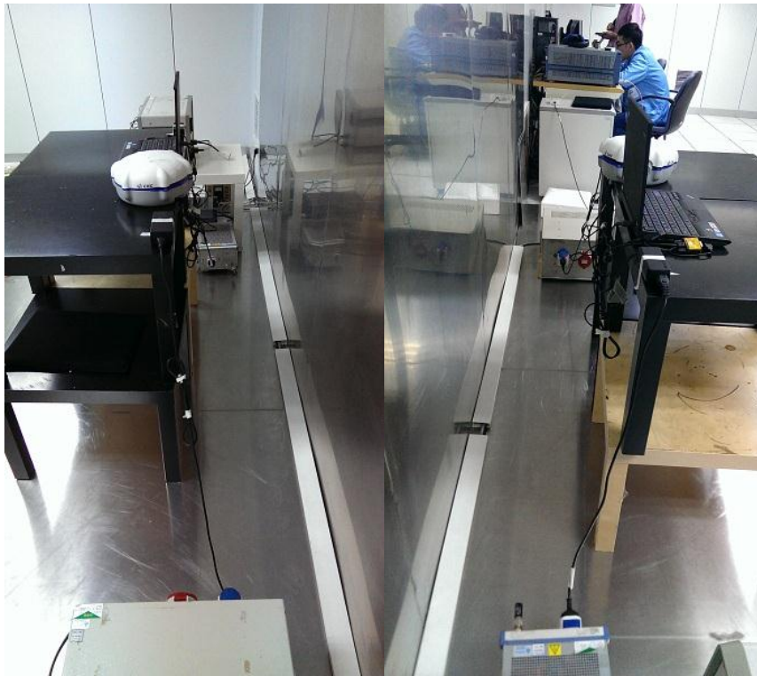
Photograph 1: Set-up for Conducted Emission, 150kHz - 30MHz
