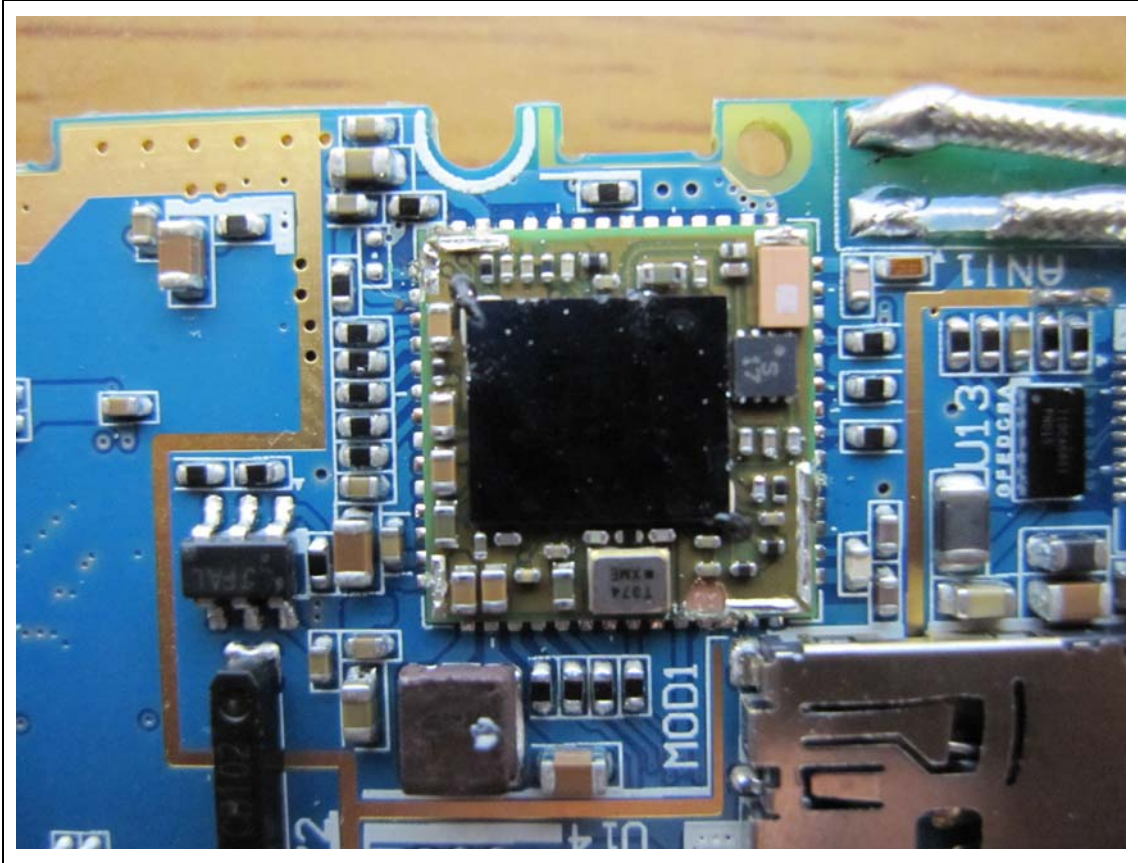
WLAN + BT module(M/N: WM-BN-BM-01) shield remove
