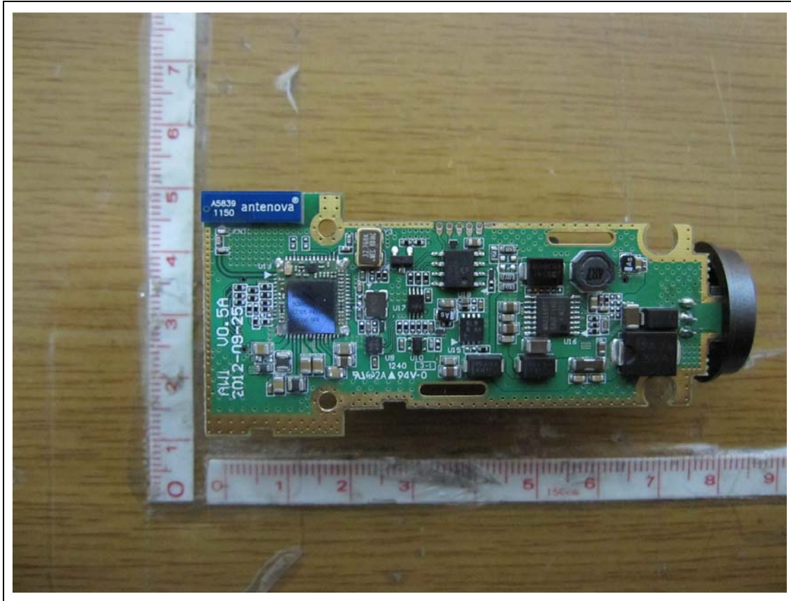
WLANBoard – Rear
