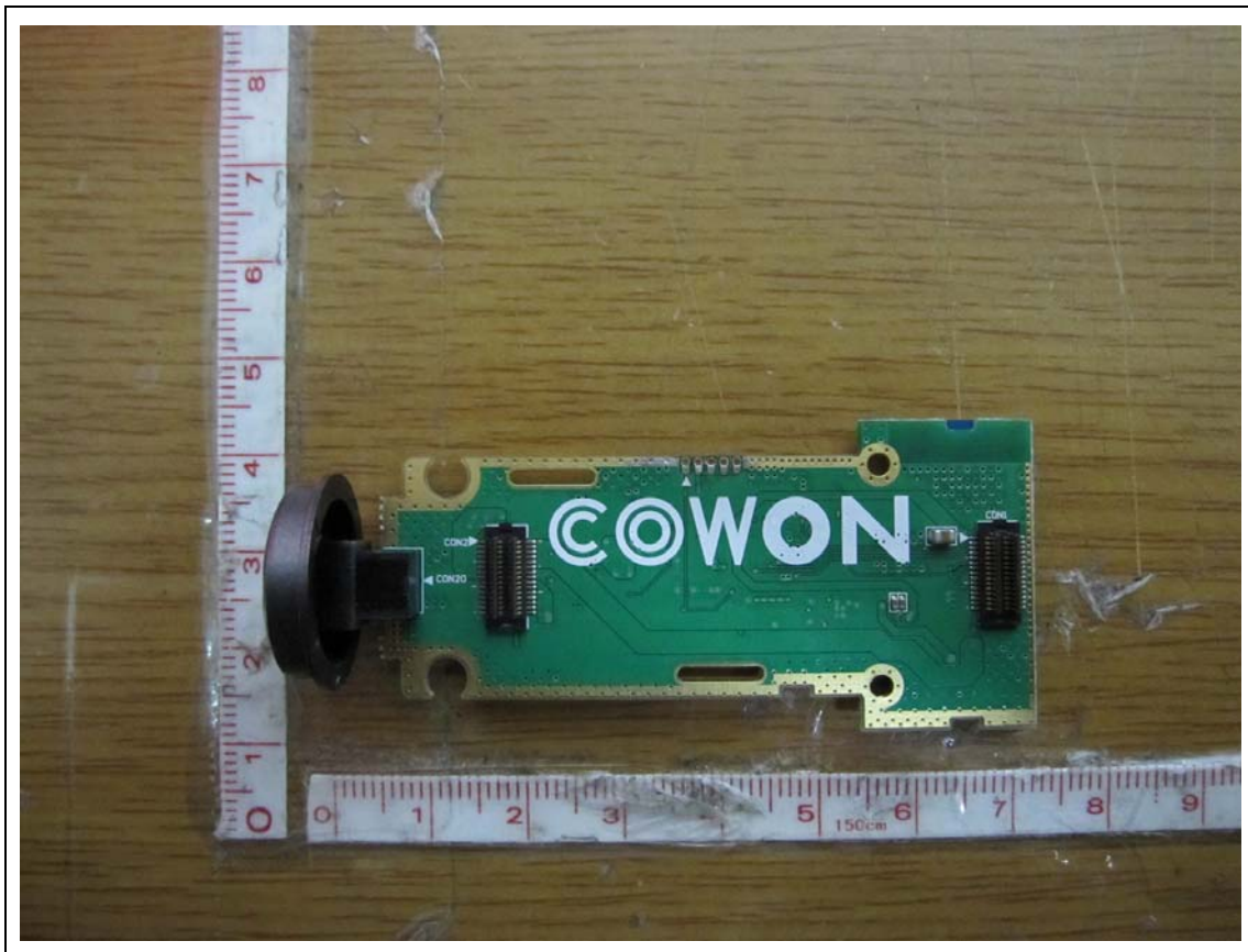
WLANBoard – Rear
