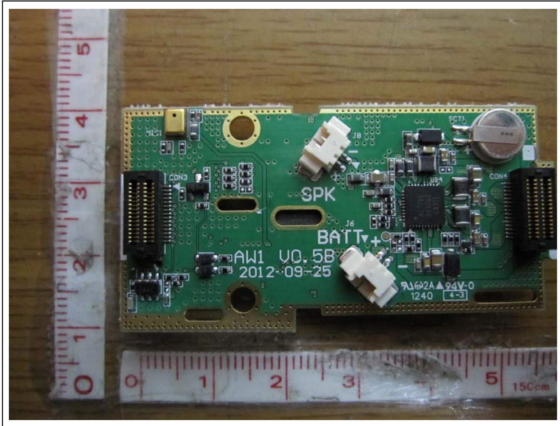
PowerBoard – Rear
