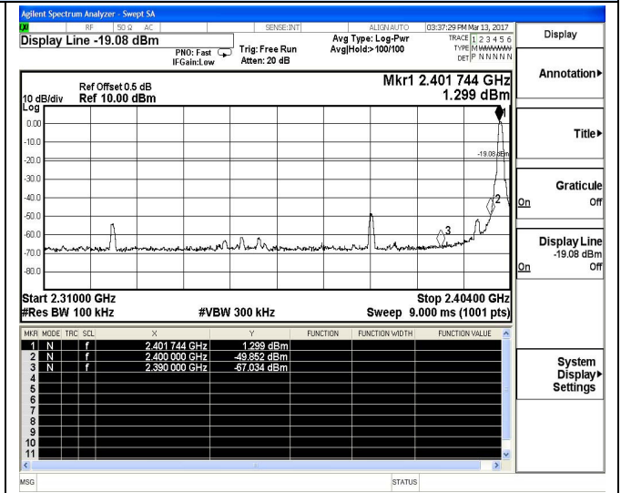
Channel 0 / 2402 MHz
