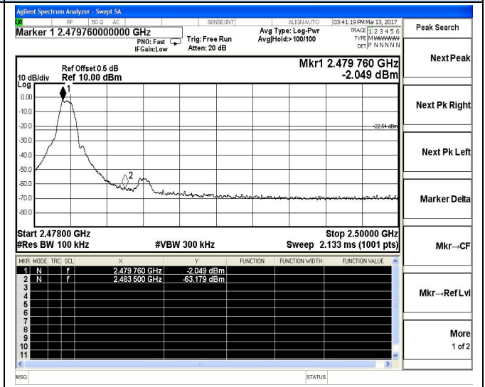
Channel 39 / 2480 MHz
