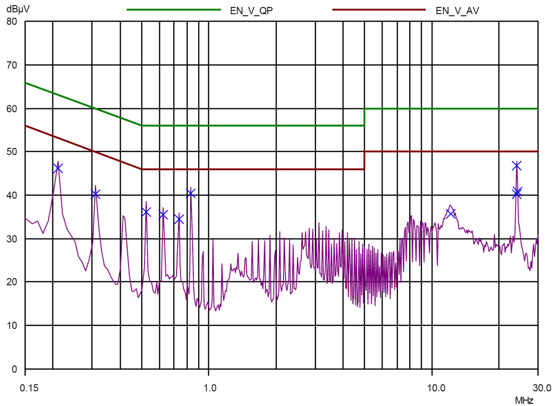
Figure 7. Plot of the Conducted Emissions
