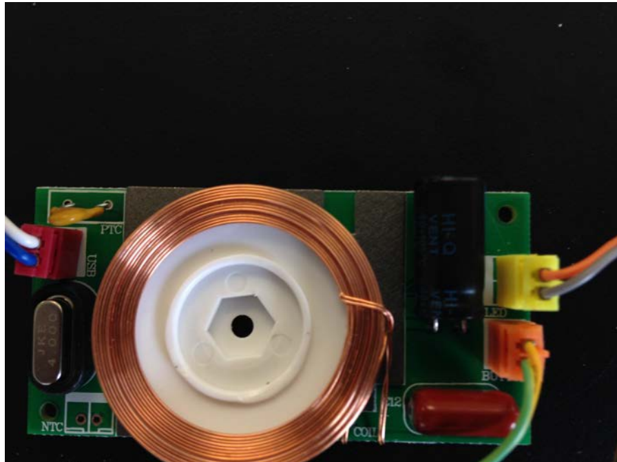
Wireless Induction Charging Cradle - Bottom
