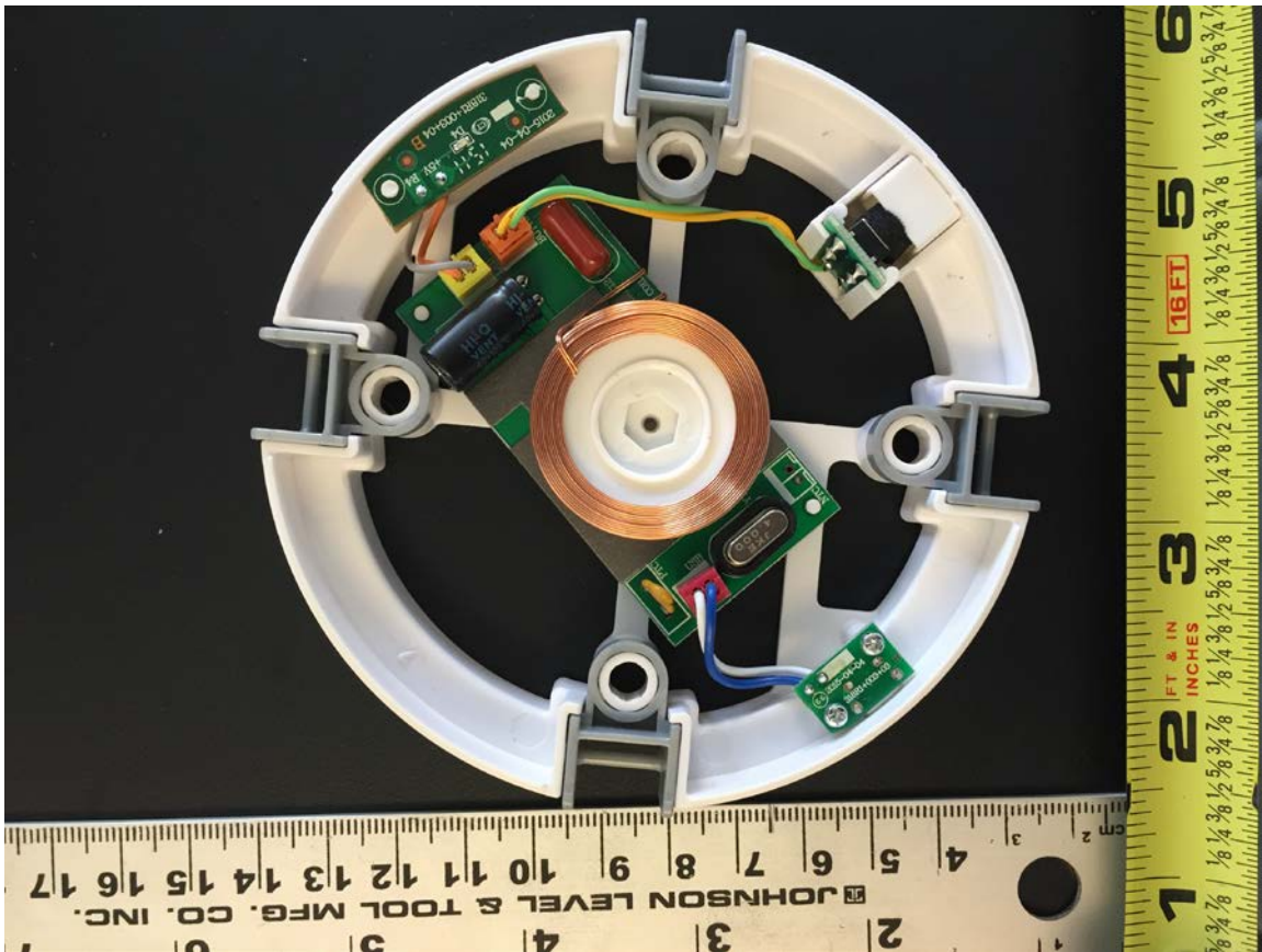
Internal View of Wireless Induction Charger – top view of internal components.
