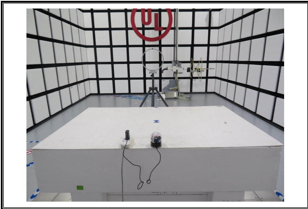
E-FILED STRENGTH MEASUREMENT SETUP FOR A POINT
