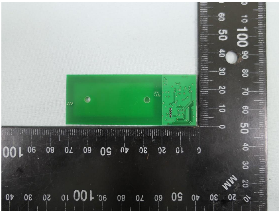
(8) EUT Photo (With RFID, Without Battery)
