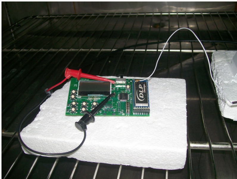
Close up of Temperature Tolerance set up (voltage variation)
