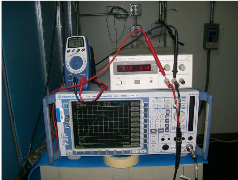
Temperature Tolerance set up (voltage variation)
