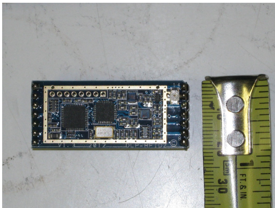
Measurement of EUT without RF Shield (view 1)
