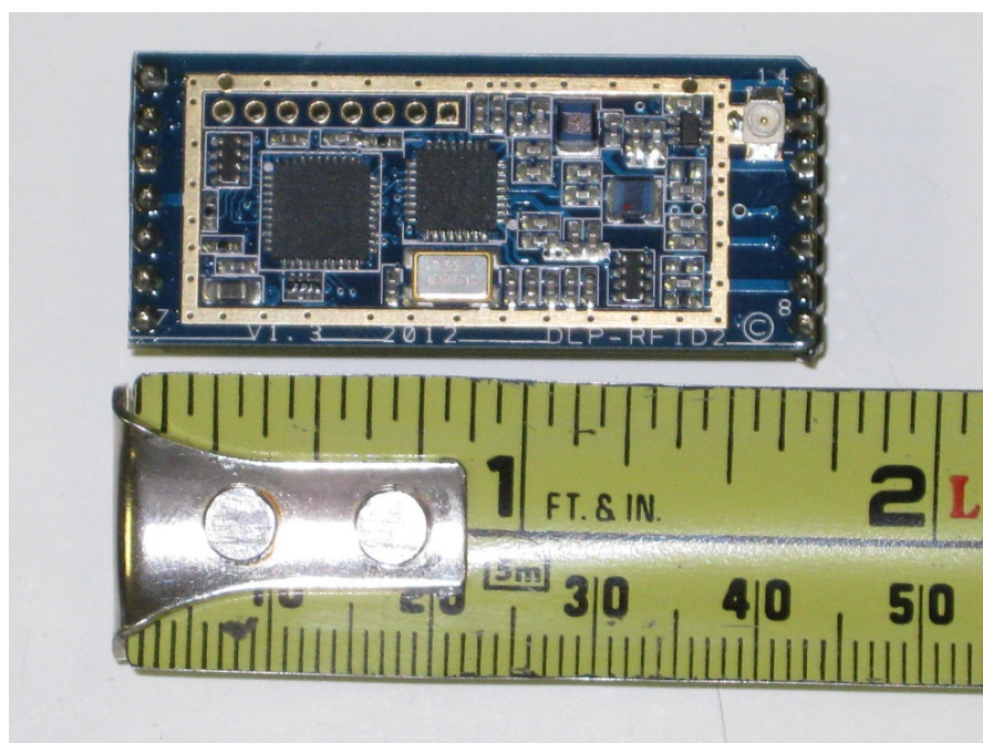
Measurement of EUT without RF Shield (view 2)
