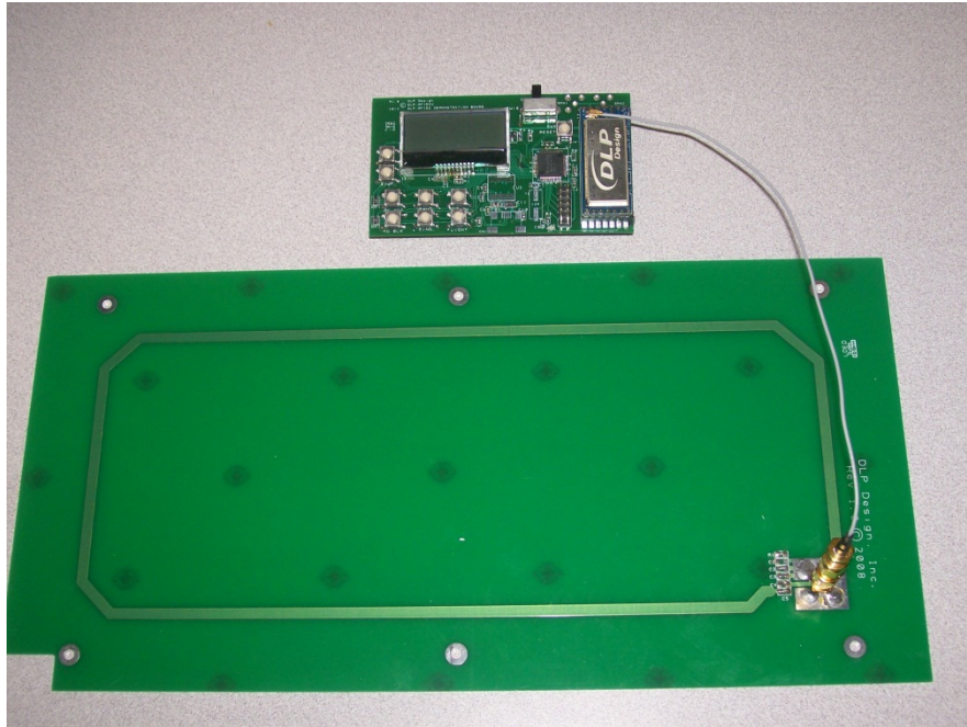
EUT with Antenna
