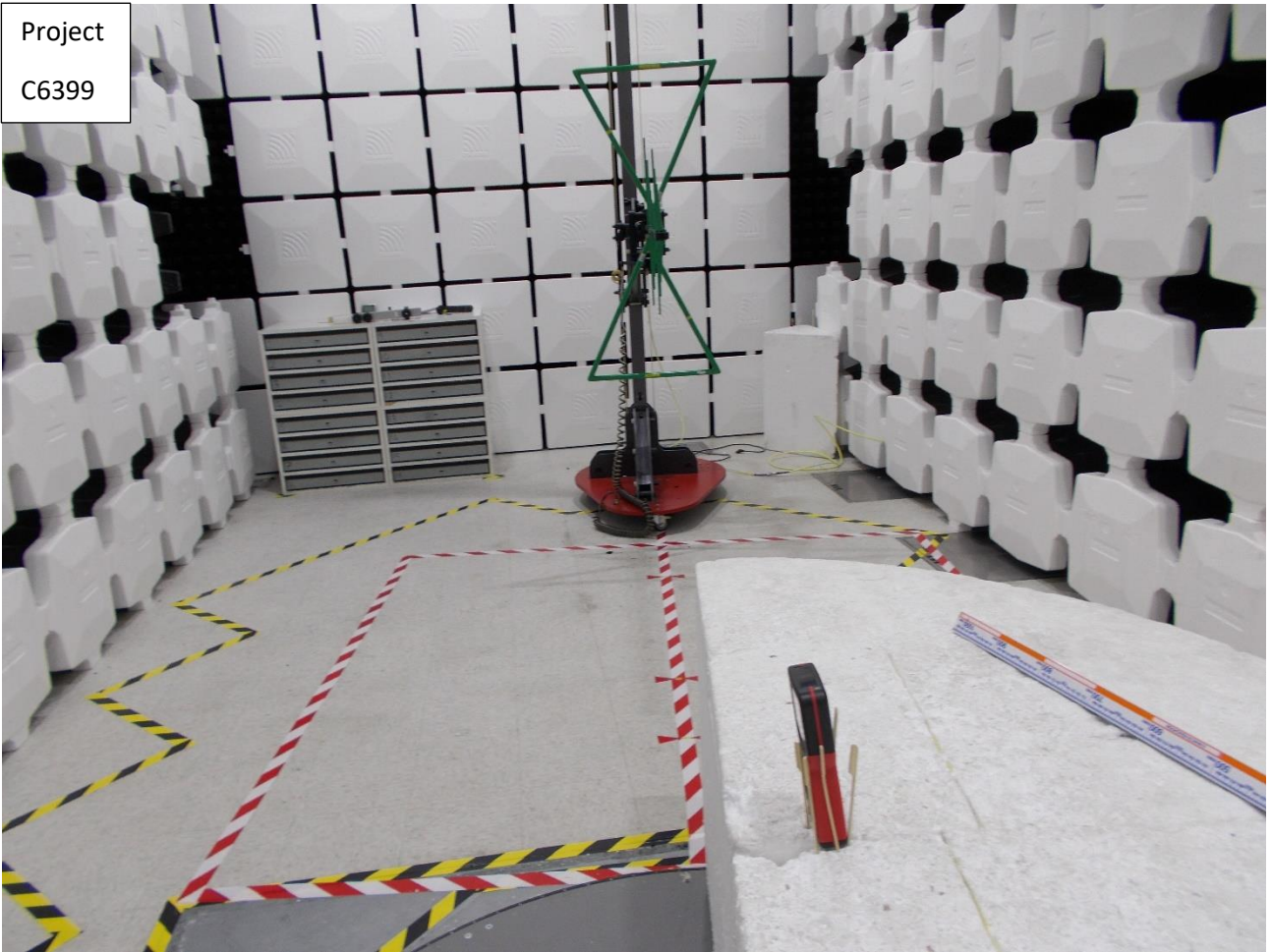
Radiated emissions 30MHz to 1GHz orientation 1
