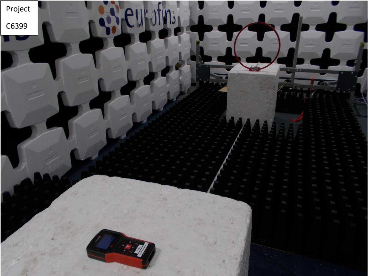
Radiated emissions 9kHz to 30MHz Orientation 3
