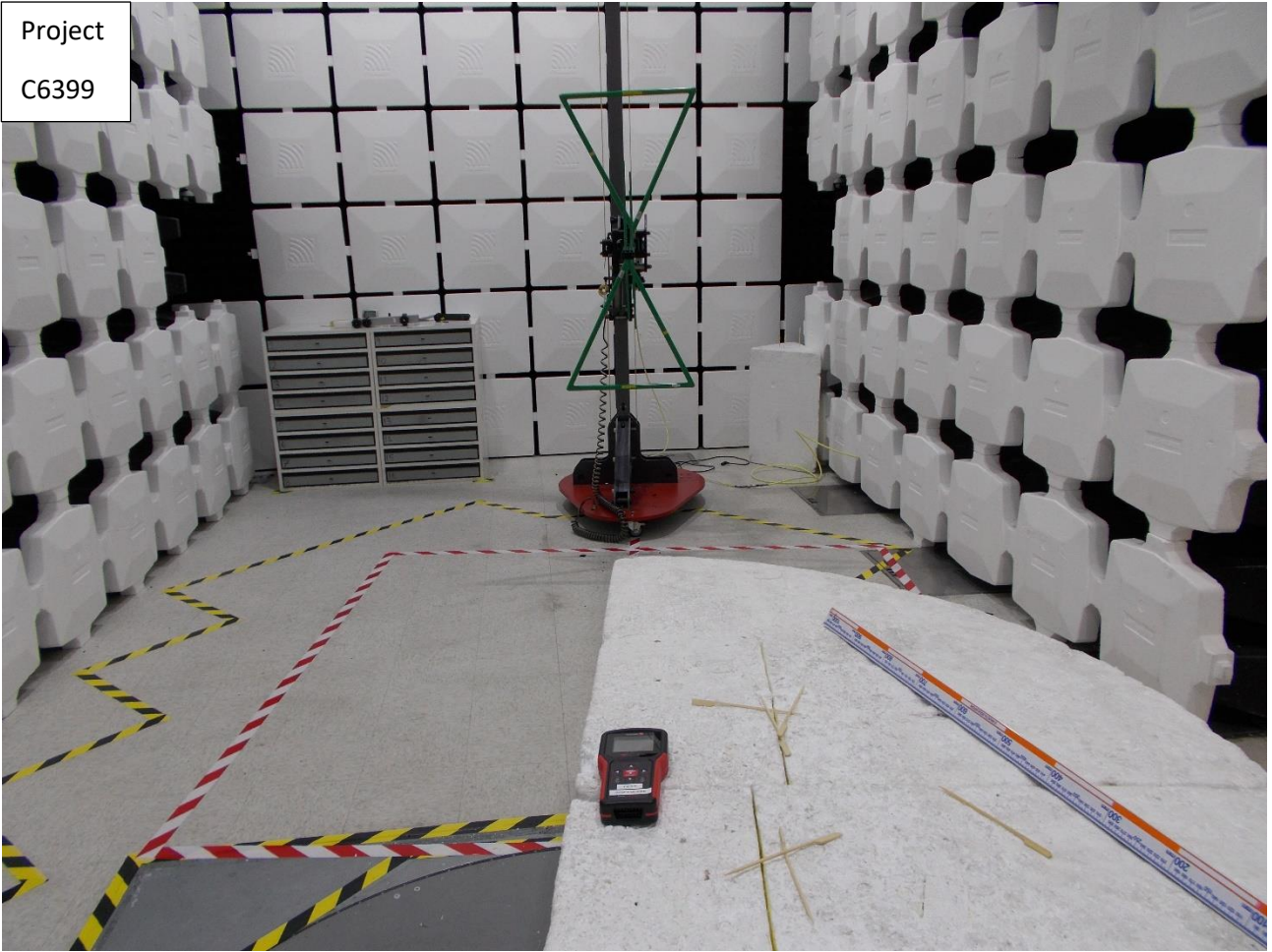
Radiated emissions 30MHz to 1GHz orientation 3
