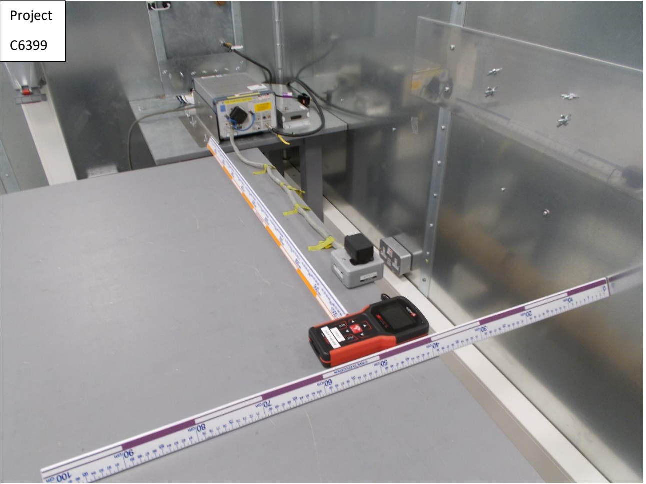
AC Mains Conducted Emissions
