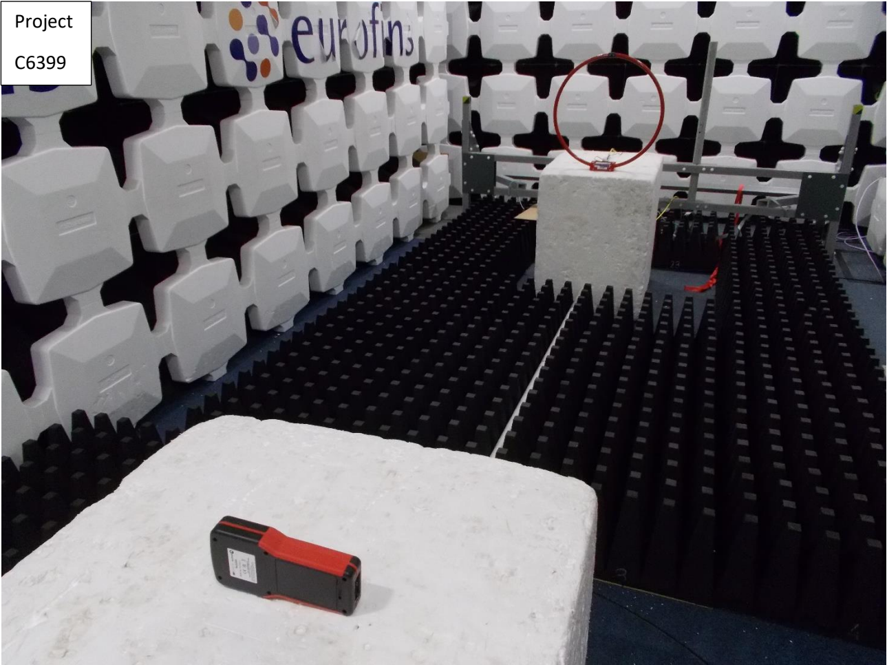
Radiated emissions 9kHz to 30MHz Orientation 2
