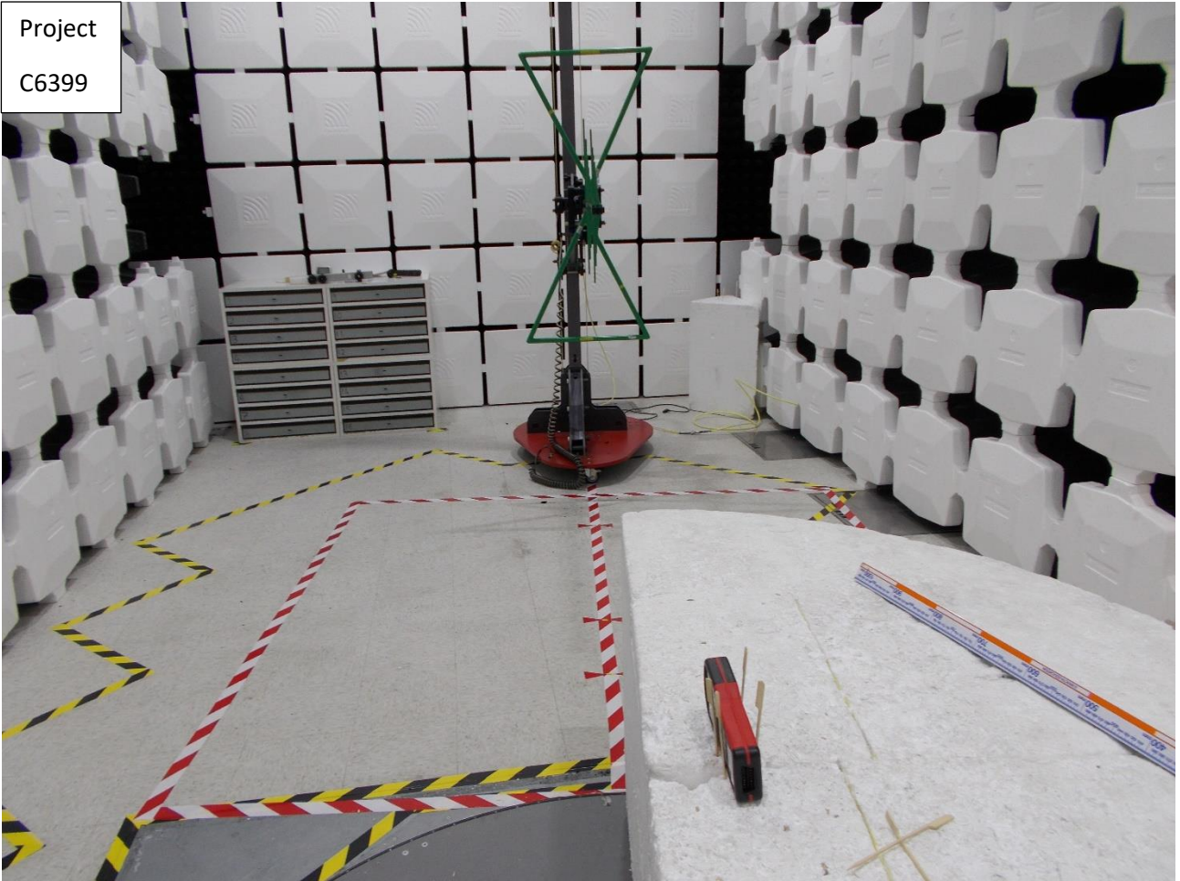
Radiated emissions 30MHz to 1GHz orientation 2
