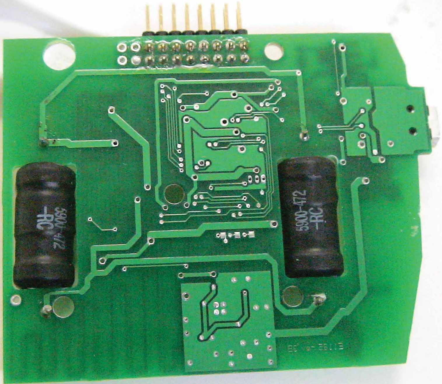
PCB (bottom)
