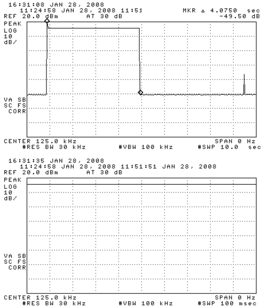
Figure 6.1(a). CW transmission modulation characteristics. (top) On time, (bottom) CW duty.
