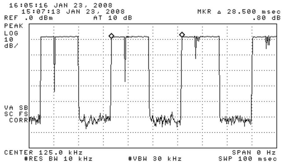
Figure 6.1(a). CW transmission modulation characteristics. (top) On time, (bottom) CW duty.
