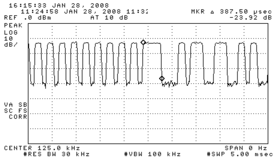
Figure 6.1(b). Worst-case modulated transmission characteristics. (first) Period, (second) Wake-up, (third) Encoding, (fourth) Data
