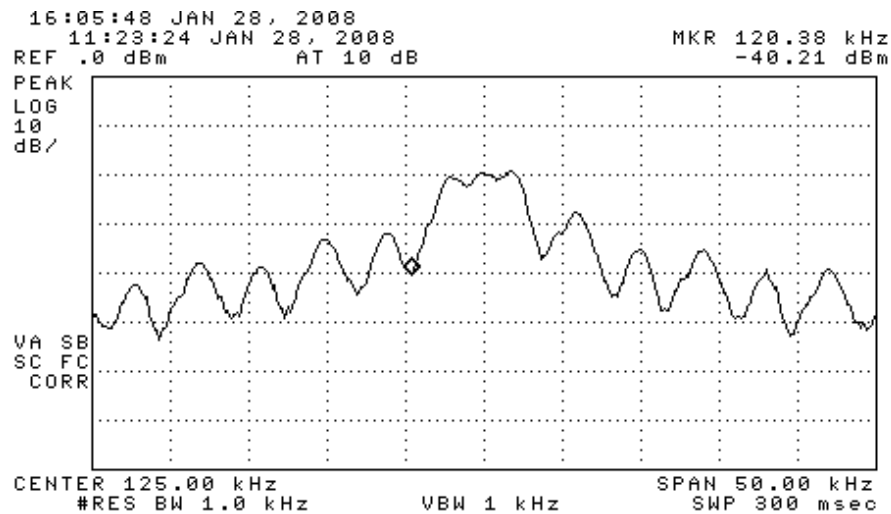
Figure 6.3. Worst Case Measured bandwidth of the DUT. (pulsed) (top) Bandwidth, (bottom) First null of sinc function.
