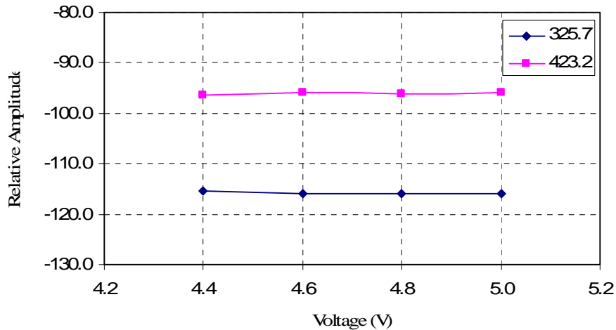
Figure 6.2. Relative emission at vs. supply voltage.
