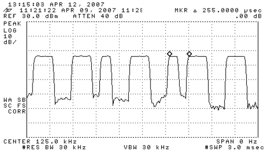
Figure 6.1. Transmission modulation characteristics. (top) Wake-up, (bottom) Manchester encoding
