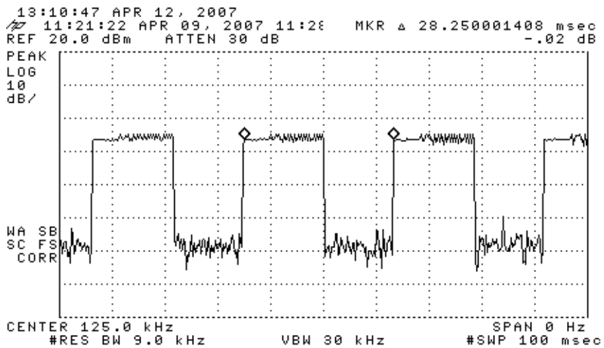
Figure 6.1. Transmission modulation characteristics. (top) CW Transmission Mode (middle) Highest data rate transmission, (bottom) modulation period
