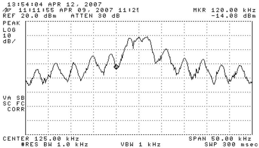
Figure 6.3. Worst case measured bandwidth of the DUT (pulsed).
