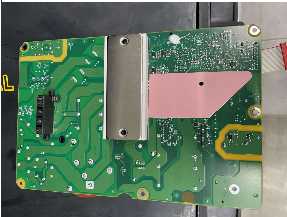
Power board Bottom:
