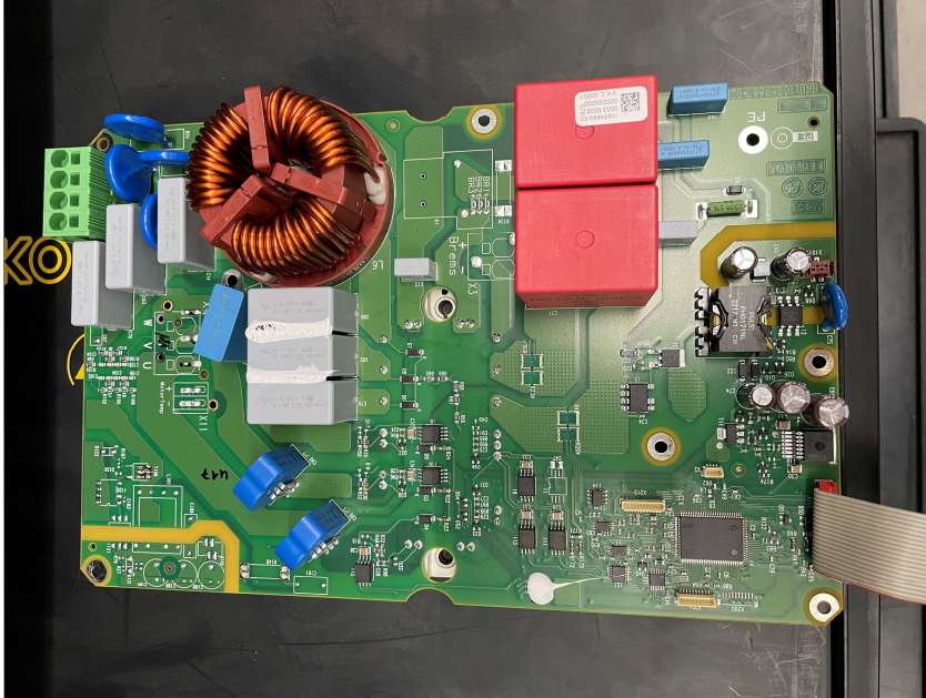
Power board Top:
