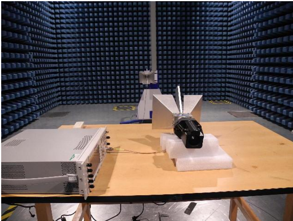
EIRP Test Setup
