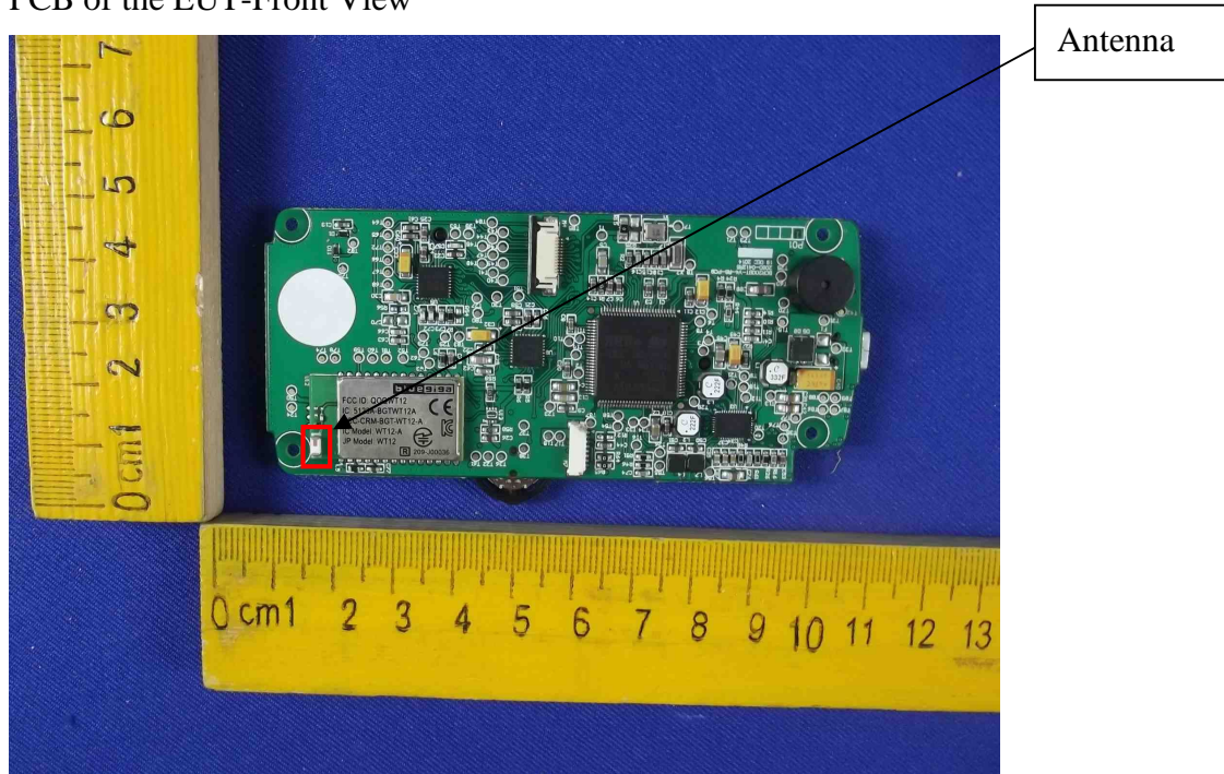
PCB of the EUT-Front View
